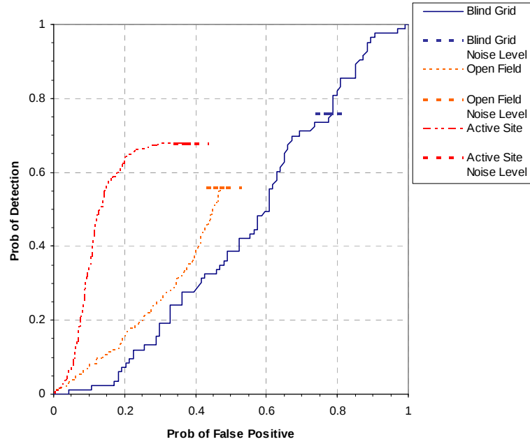
Figure 4. EM63/PUSHCART P_d^{\text{res}} stages versus the respective P_{\text{fp}} over all ordnance categories combined.
