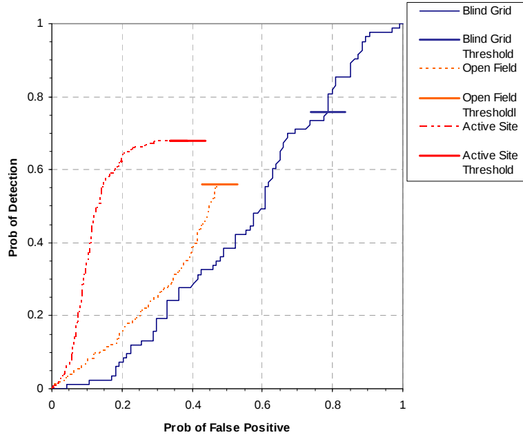
Figure 5. EM63/PUSHCART P_d^{\text{disc}} versus the respective P_{\text{fp}} over all ordnance categories combined.
