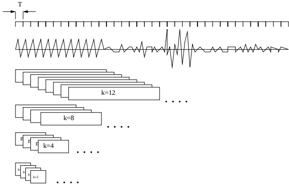
Fig. 2. Illustration of some of the processing windows that need to be computed as input to the MRHMM. In all, it is necessary to compute all window sizes at all start times for each state.
