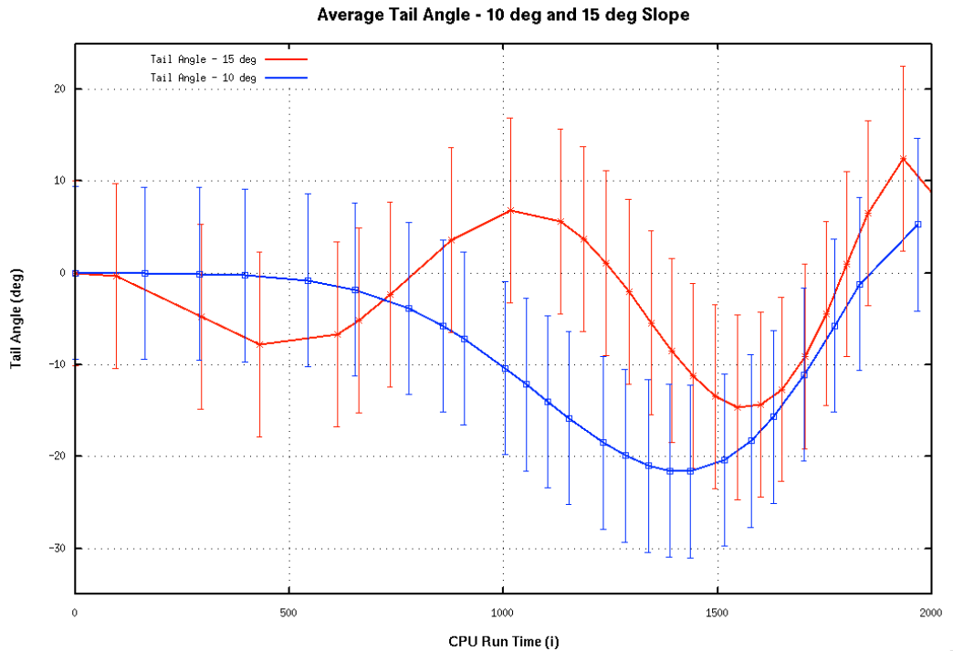
Figure 40. Average Tail Angle – 10° and 15°
