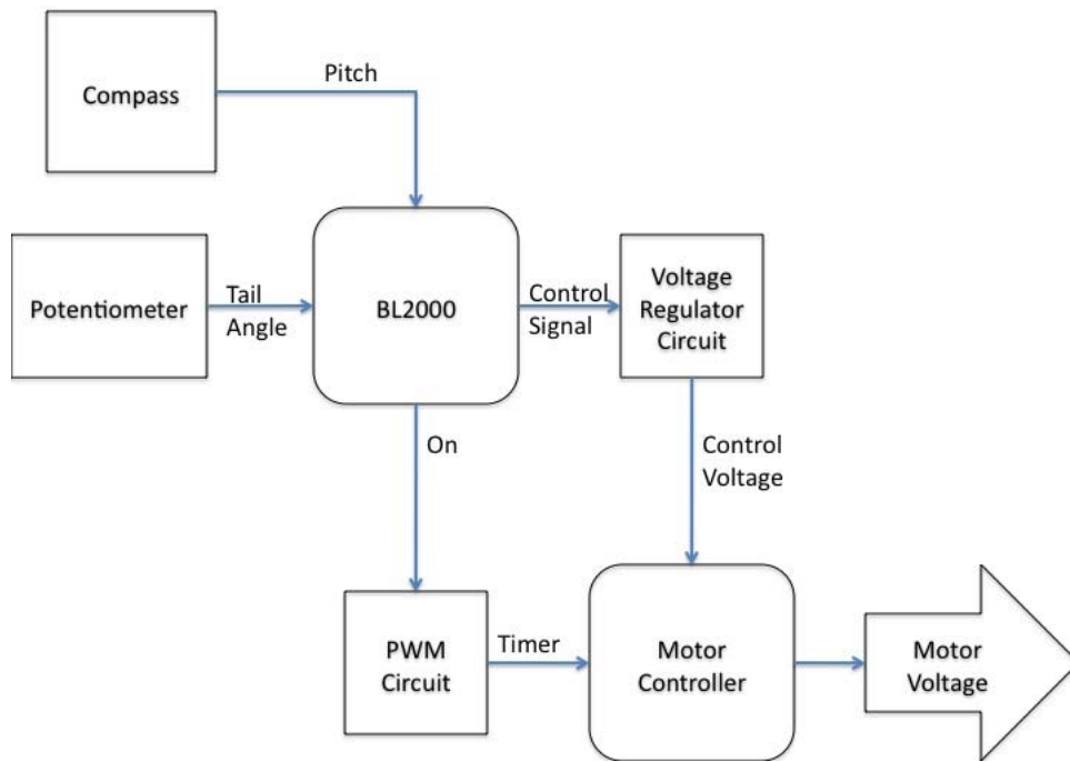
Figure 12. Tail Component Functional Diagram
