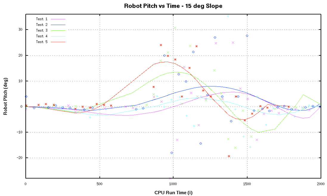
Figure 35. Robot Pitch vs. Time - 15^\circ
