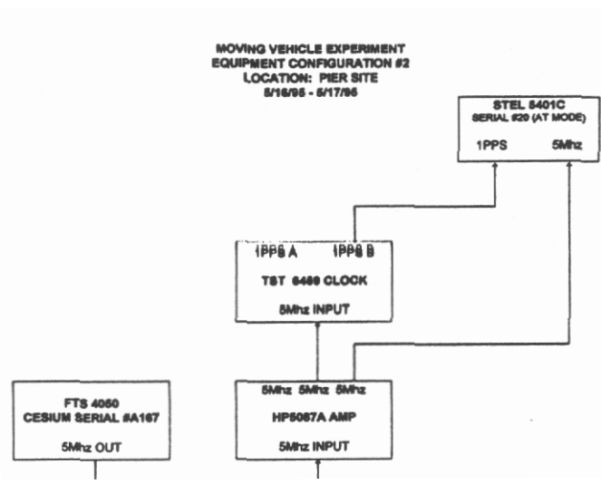
Figure 3 - Final Equipment Configuration at Pier Site
