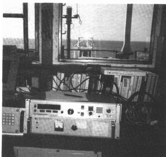
Photo 9 - Equipment in Bridge on RV Ranger
