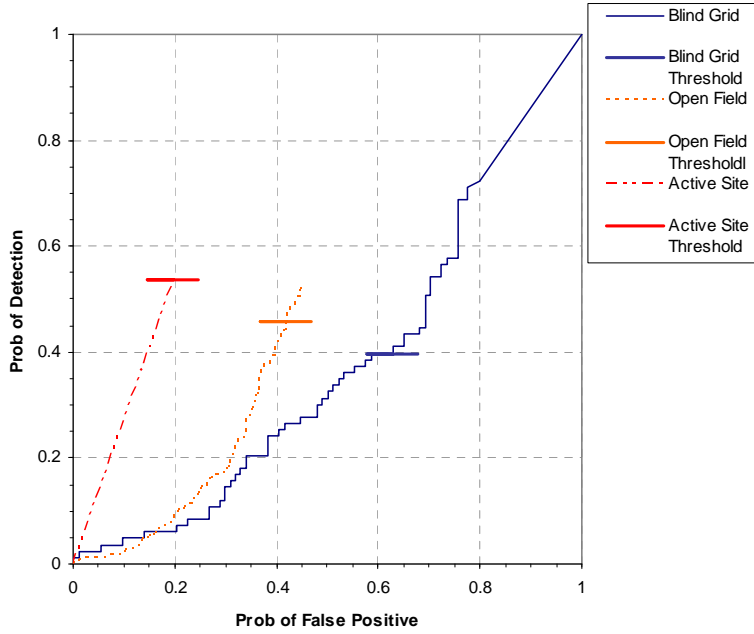
Figure 7. Dual mode STOLS/towed array P_d^{\text{disc}} versus the respective P_{\text{fp}} over all ordnance categories combined.
