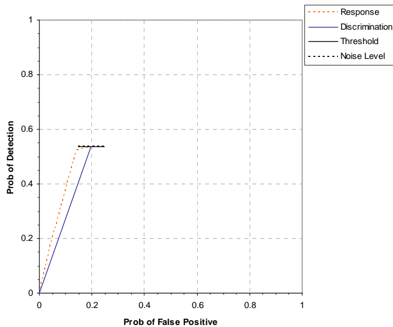
Figure 2. Dual mode STOLS/towed array active response P_d^{\text{res}} and P_d^{\text{disc}} versus their respective P_{\text{fp}} over all ordnance categories combined.
