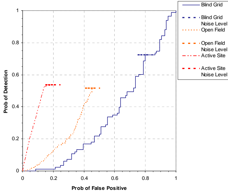
Figure 6. Dual mode STOLS/towed array P_d^{\text{res}} stages versus the respective P_{\text{fp}} over all ordnance categories combined.
