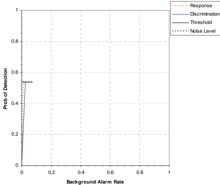
Figure 3. Dual mode STOLS/towed array active response P_d^{\text{res}} and P_d^{\text{disc}} versus their respective BAR over all ordnance categories combined.
