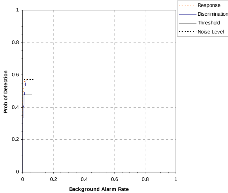
Figure 3. GEM-5/TOWED ARRAY active response P_d^{\text{res}} and P_d^{\text{disc}} versus their respective BAR over all ordnance categories combined.
