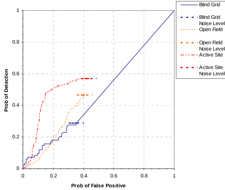
Figure 6. GEM-5/TOWED ARRAY P_d^{\text{res}} stages versus the respective P_{\text{fp}} over all ordnance categories combined.
