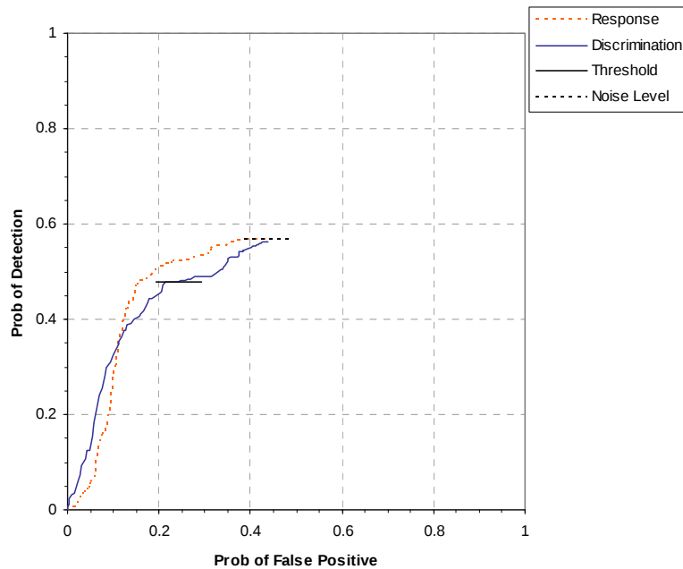
Figure 2. GEM-5/TOWED ARRAY active response P_d^{\text{res}} and P_d^{\text{disc}} versus their respective P_{\text{fp}} over all ordnance categories combined.
