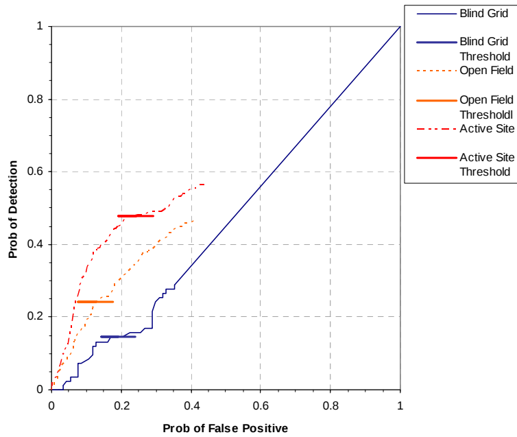
Figure 7. GEM-5/TOWED ARRAY P_d^{\text{disc}} versus the respective P_{\text{fp}} over all ordnance categories combined.
