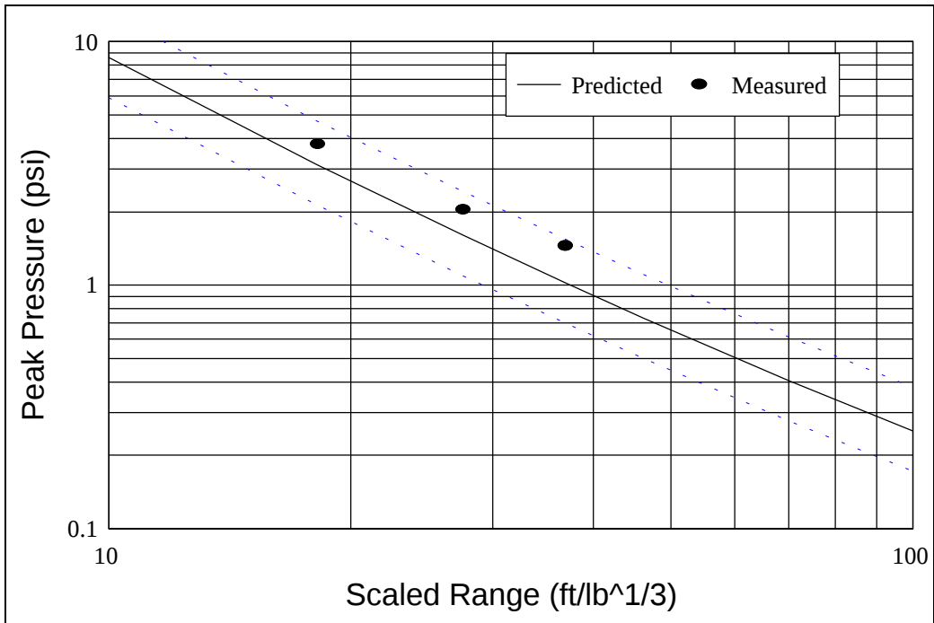
Figure 24. Measured vs. predicted peak external pressures: Front.
