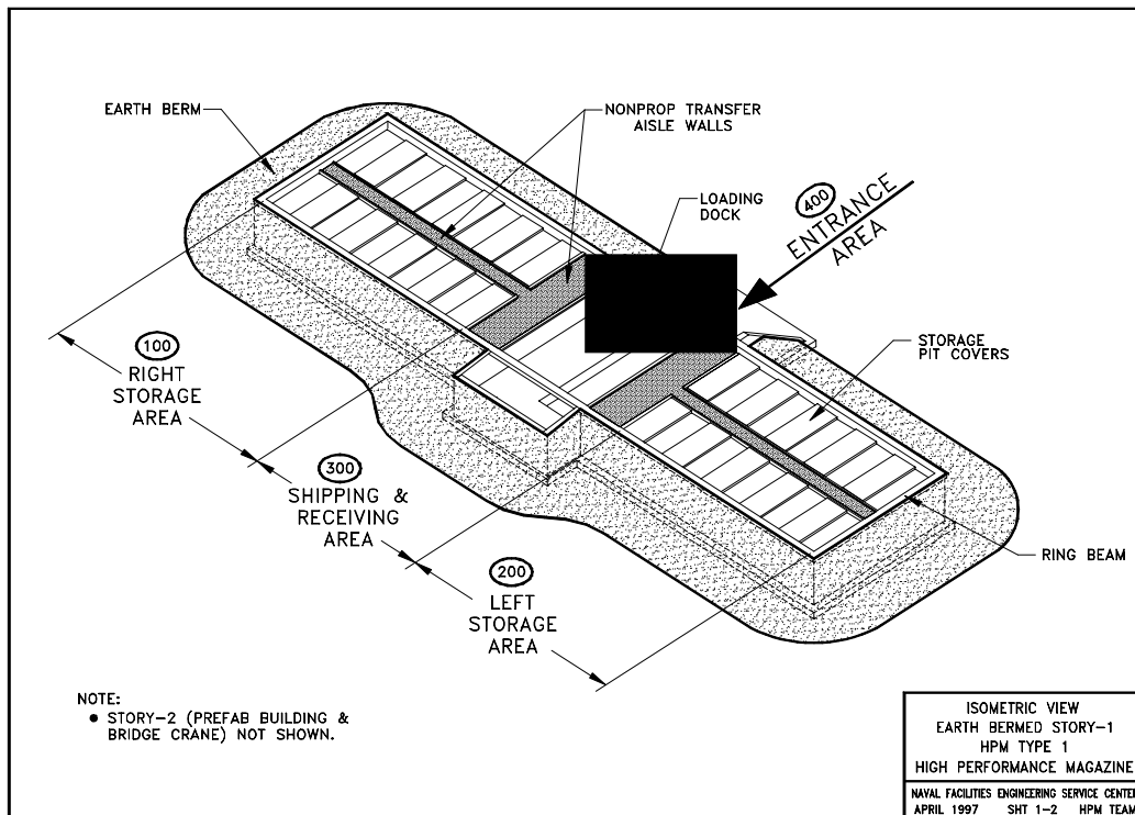
Figure 2. High Performance Magazine: Isometric view of Story-1.
