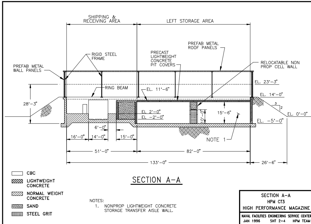
Figure 7. CT3 structure: Section A-A.
