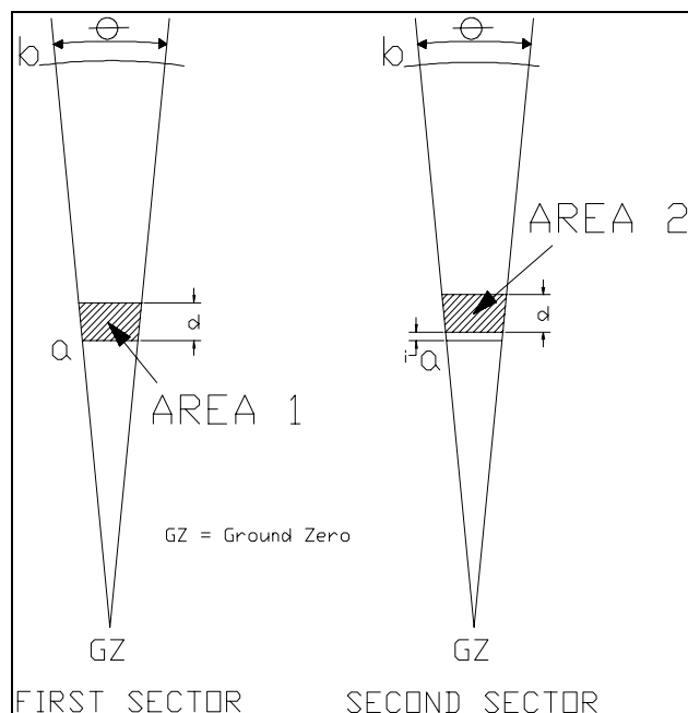
Figure 27. Schematic representation of Jacobs' Method.
