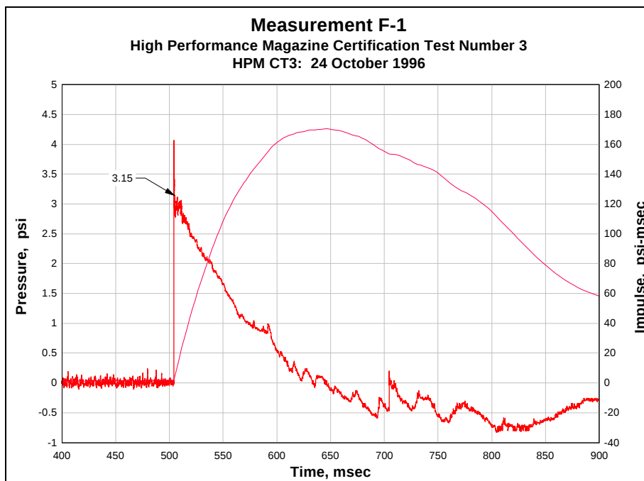
Figure 23. External airblast pressure measurement F-1.
