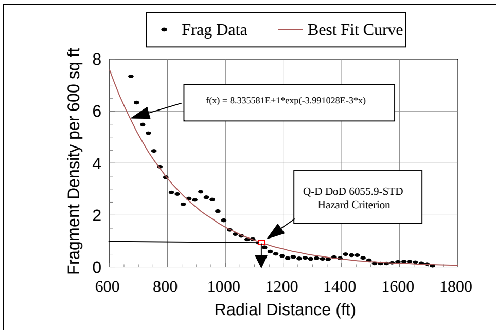
Figure 29. Debris areal number density distribution: Side sector.
