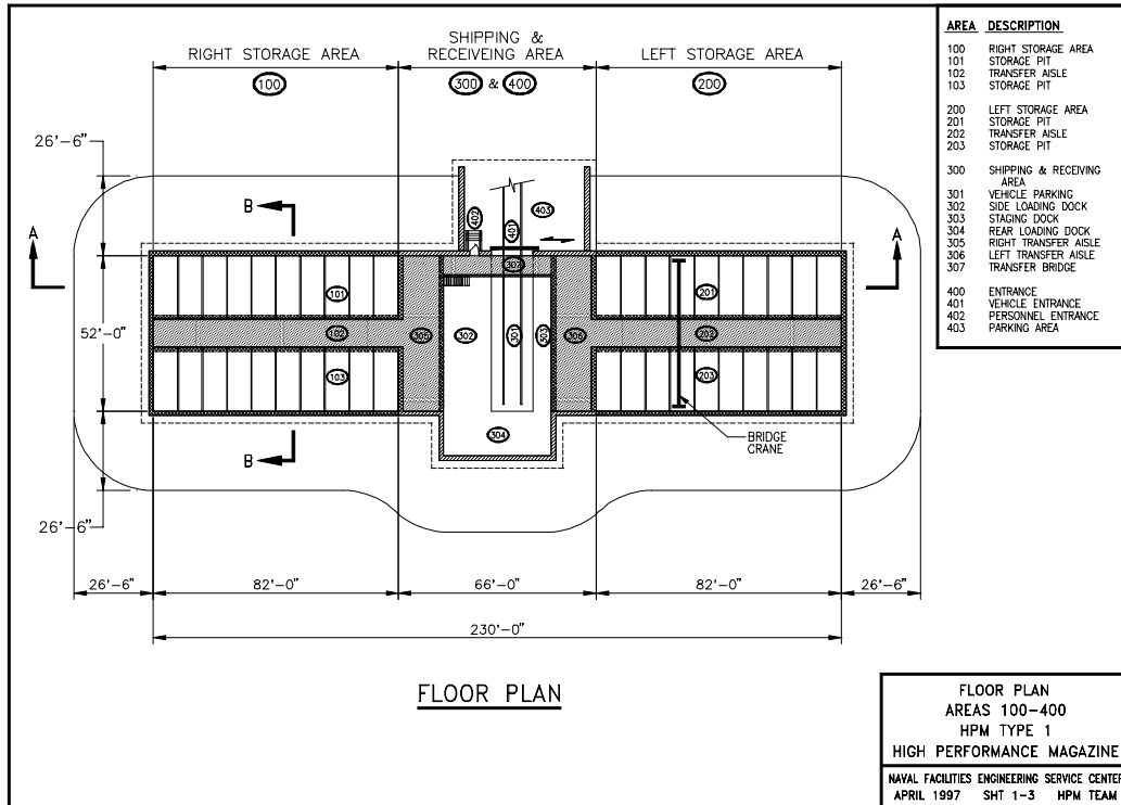
Figure 3. High Performance Magazine: Floor plan.
