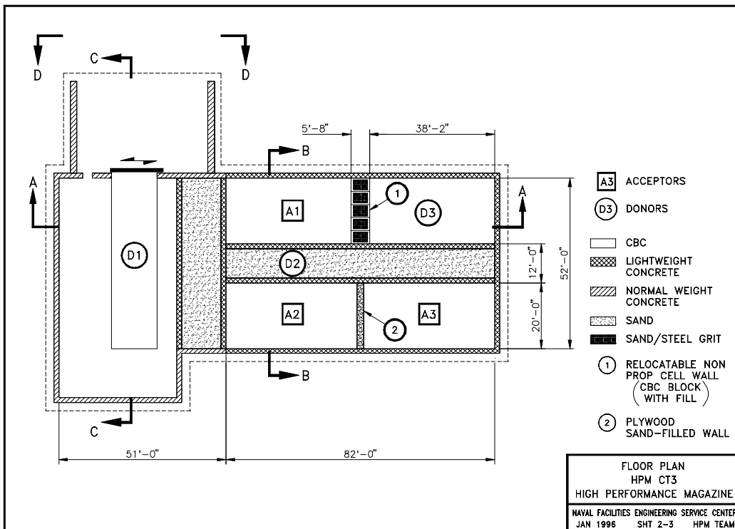
Figure 6. CT3 structure: Floor plan.
