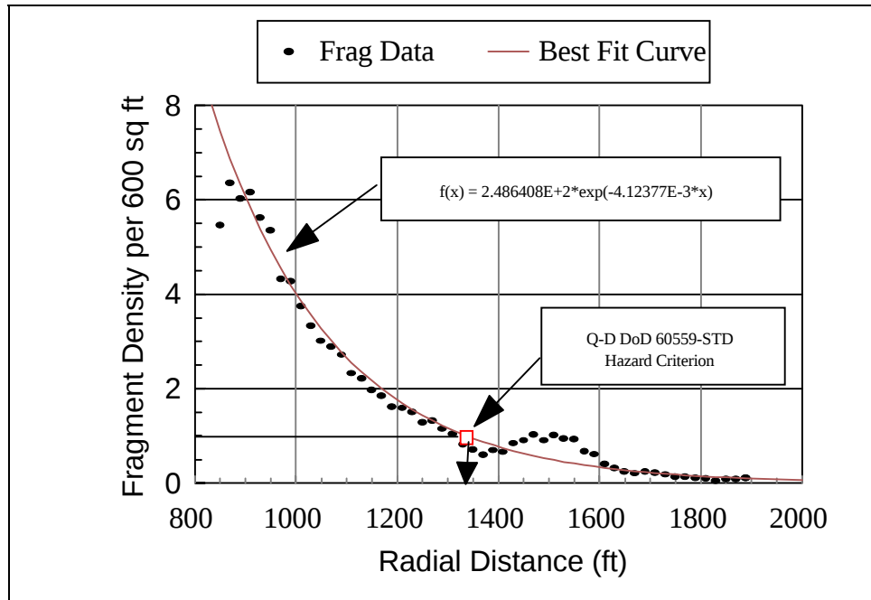
Figure 28. Debris areal number density distribution: Front sector.
