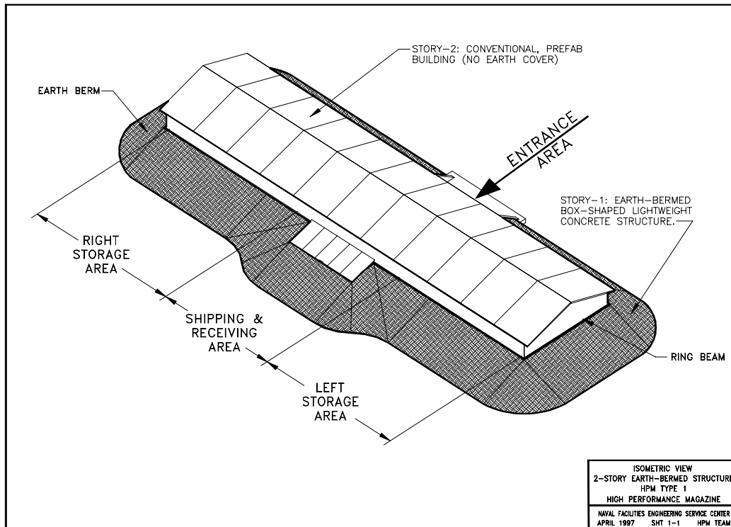
Figure 1. High Performance Magazine: Isometric view of magazine.
