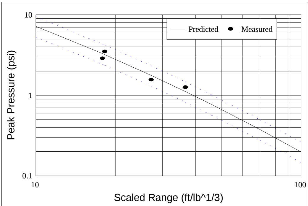
Figure 25. Measured vs. predicted peak external pressures: Side & Back.
