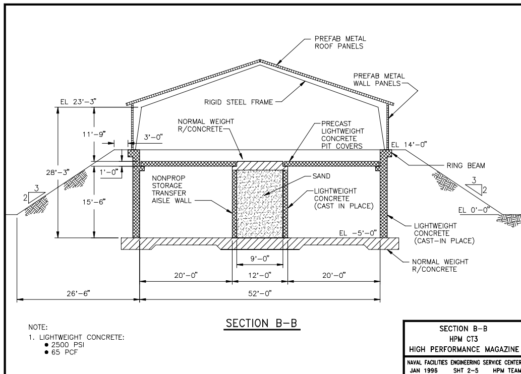
Figure 8. CT3 structure: Section B-B.
