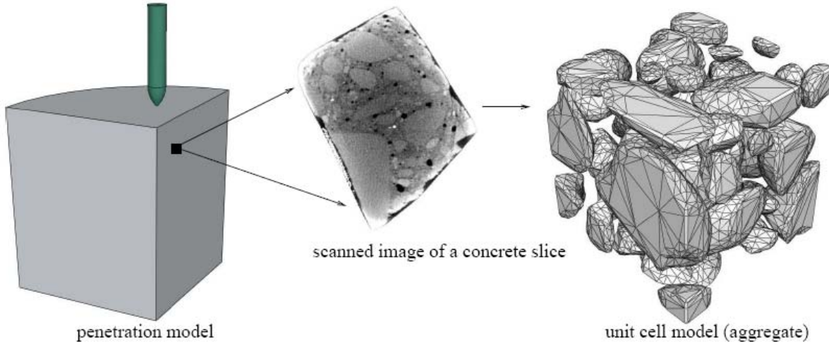
Figure 6. Construction of the unit cell model from digital image of concrete sample
