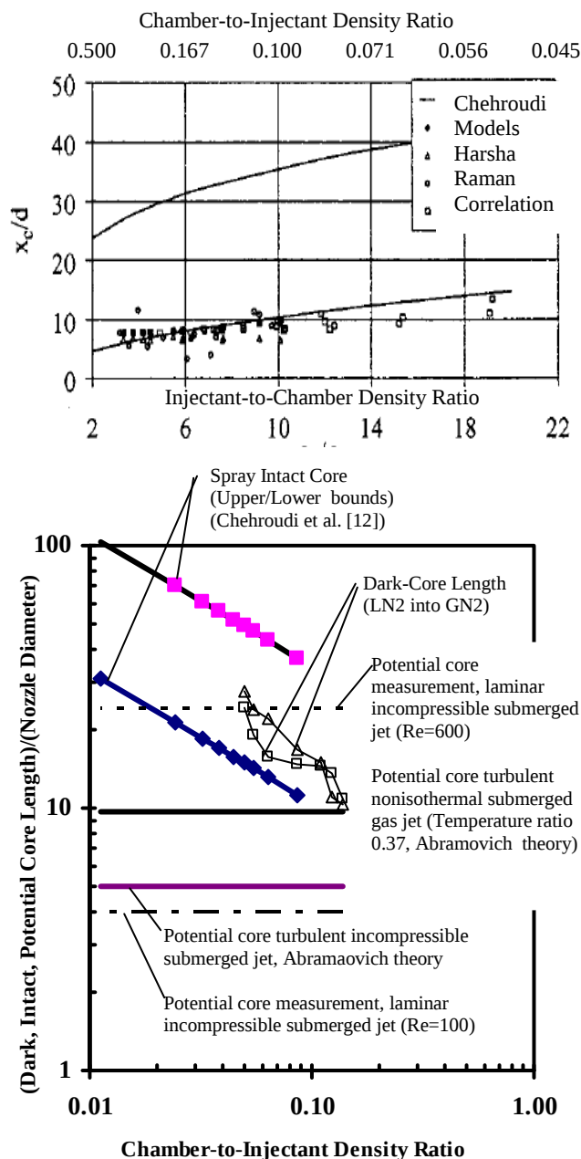
Figure 7. Comparison of the mean dark core length measurements for \text{LN}_2 jet injection into \text{GN}_2 at room temperature from sub- up to supercritical pressures. Also, shown are boundaries using Chehroudi's (intact) core equation (solid diamond and square symbols). Note that the horizontal axis of the two plots are inverse of each other. Chehroudi et al. [20] and Oschwald et al. [21].
