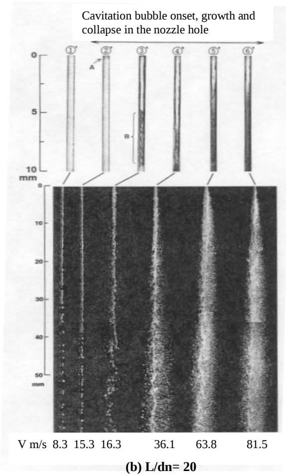
Figure 11 (a & b). Internal flow in the nozzle hole and disintegration behavior of the liquid jets (effects of L/dn ). The breakup length measured by the Hiroyasu's group as a function of injection velocity is shown. It is indicated, for example, that when cavitation bubbles form but collapse inside the injector, enhanced atomization and consequently shorter breakup lengths are achieved. However, when a hydraulic flip occurs, it tends to increase the breakup length. V is injector velocity. Tamaki et al. [23].
