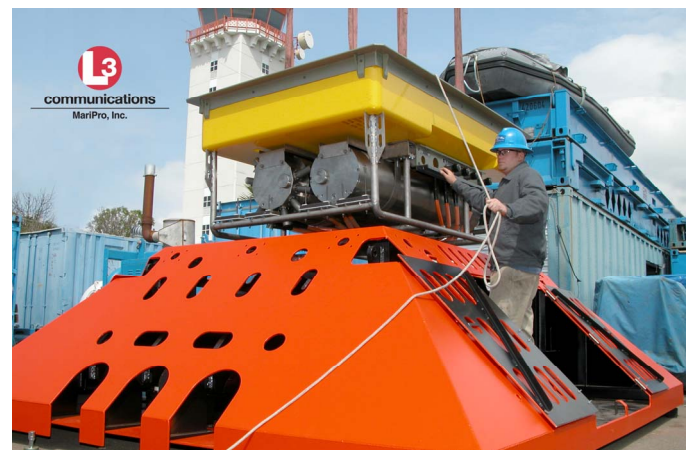
Figure 4. MARS Science Node (photo courtesy of MariPro, Inc.)
