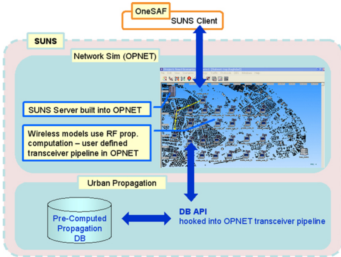
Fig. 1. SUNS Architecture.
