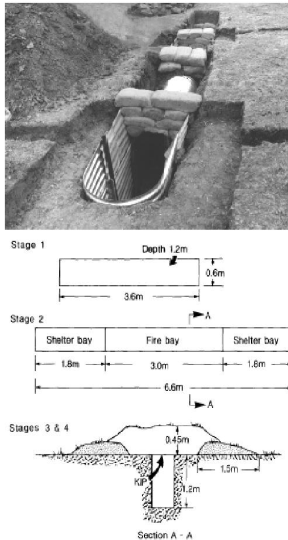
Figure 4A-4-1: Four-Man Battle Trench (One Type that Has Been Used by the British Army).
