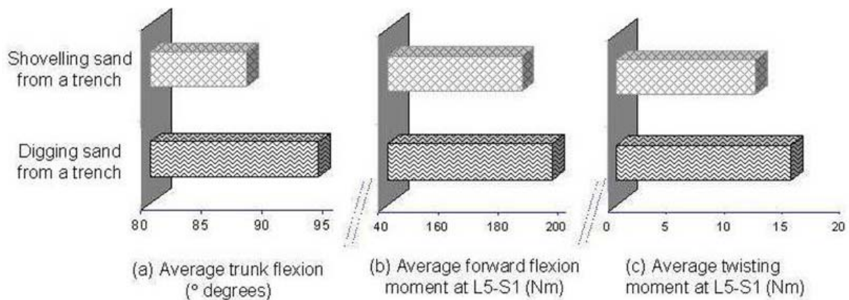
Figure 4-2: Data Reported by Van der Grinten 1987 for Digging and Shovelling Sand from Trenches (at the beginning of the lifting action): (a) Average forward flexion of the trunk; (b) average moment in the lower back at L5-S1; and (c) average twisting moment at L5-S1.
