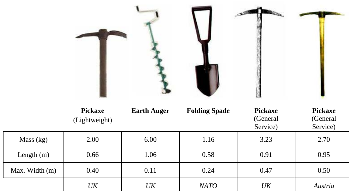
Figure 4-7: Equipment Used to Break or Loosen Ground Material within the Armed Forces of NATO.
