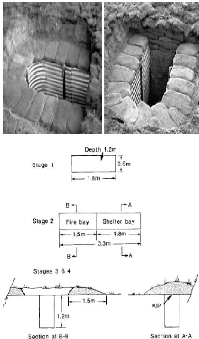
Figure 4A-3-1: Two-Man Battle Trench (One Type that Has Been Used by the British Army).
