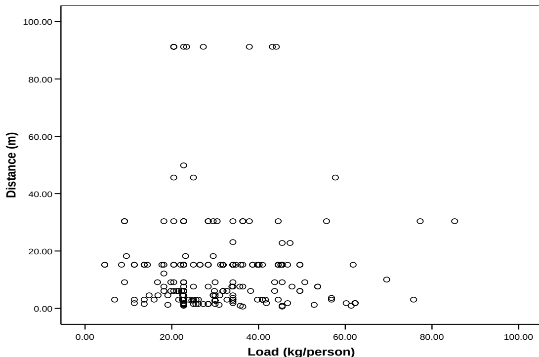
Figure 5-3: Relationship Between Load and Distance Carried for US Army Lifting and Carrying Tasks.
