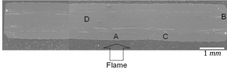
Figure 77: Polished section from heated zone of runout prepreg MI Hi-Nic-S/BN/SiC fatigued at 105 MPa
