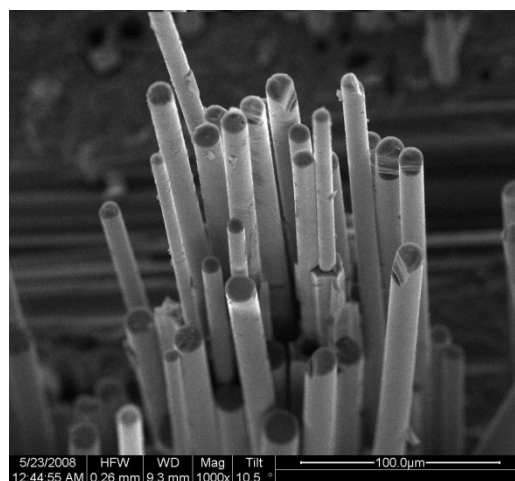
Figure 66: Microstructure of fatigued tested specimen under peak stress of 66% of PL: I and J are from the oxidized, and K and L are from the non-embrittled region of the fracture surface. Specific locations imaged are shown on Figure 62.
