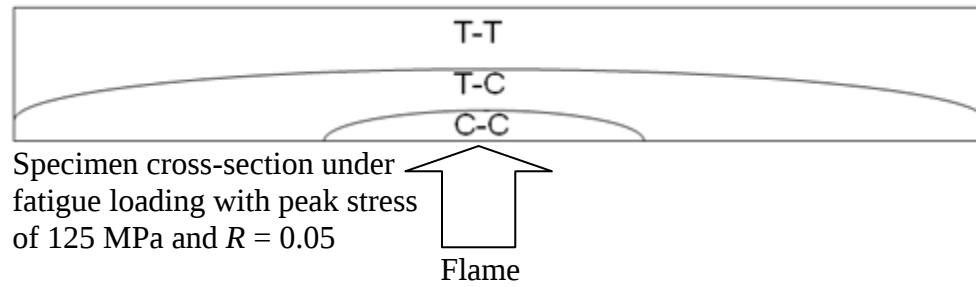
Figure 111: Illustration of varying stress states on a cross-section due to thermal gradient stress
