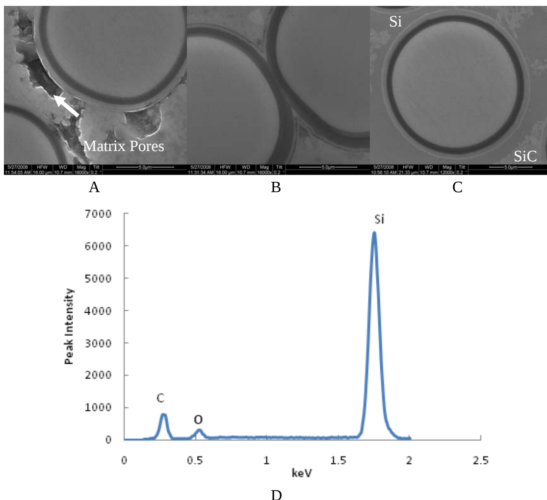
Figure 79: Gradient nature of pores in MI matrix; (A) 1 st ply, (B) 4 th ply, (C) 8 th ply from impinging surface; (D) EDS in the porous area indicated in (A)
