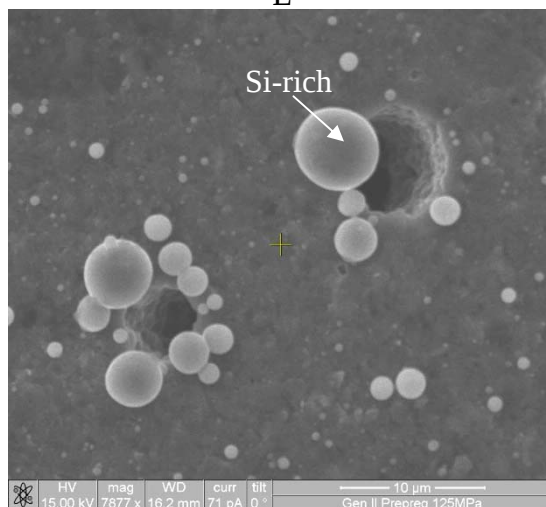
Figure 74: Microstructure of the MI prepreg Hi-Nic-S/BN/SiC fatigued at peak stress of 56% of PL : E thru H are from the fracture surface as shown on Figure 72.
