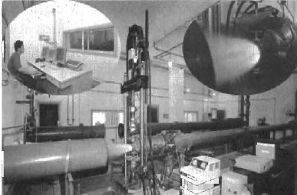
Figure 9: Wind tunnel experimental system at Northwestern Polytech University in China
