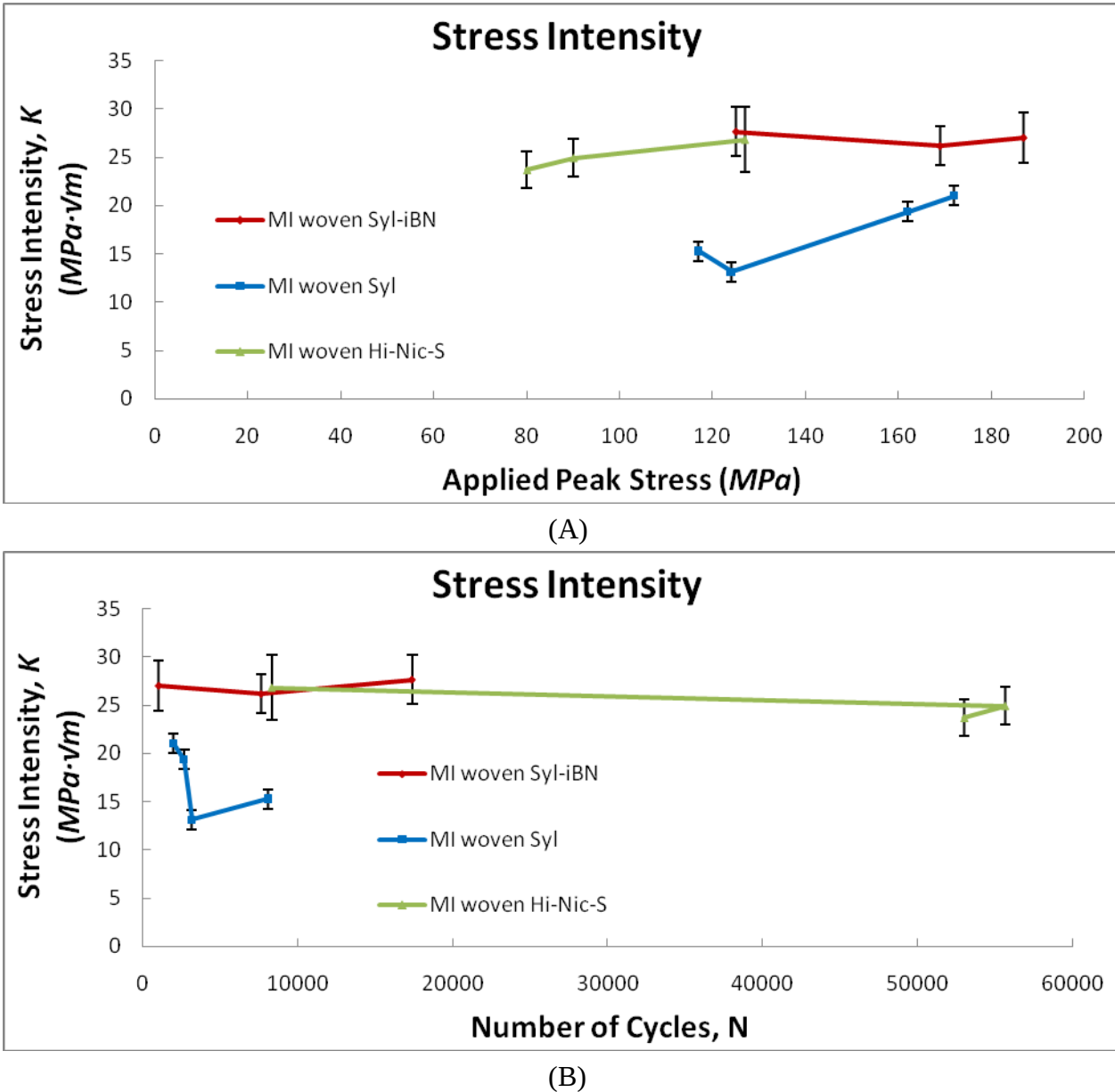
Figure 125: Stress Intensity plotted with respect to.(A) applied peak stress and (B) number of cycles
