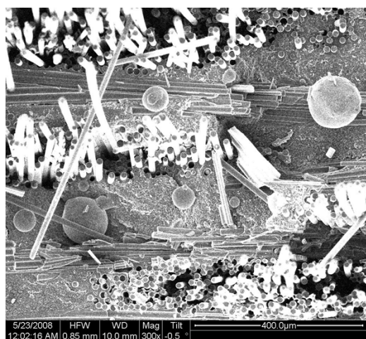
Figure 66: Microstructure of fatigued tested specimen under peak stress of 66% of PL: I and J are from the oxidized, and K and L are from the non-embrittled region of the fracture surface. Specific locations imaged are shown on Figure 62.
