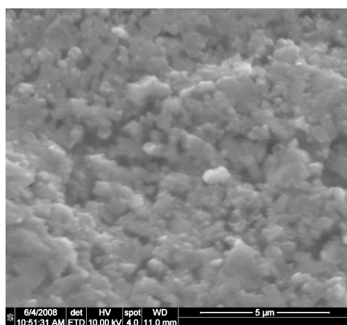
Figure 115: Matrix recession in all four CMCs: (A) woven MI Syl-iBN/BN/SiC, (B) woven MI Syl/BN/SiC, (C) woven MI Hi-Nic-S/BN/SiC and (D) prepreg MI Hi-Nic-S/BN/SiC
