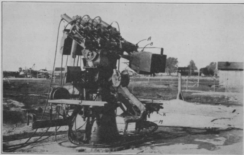
FIG. 10. MULTIPLE MOUNT FOR 50-CALIBER MACHINE GUNS
