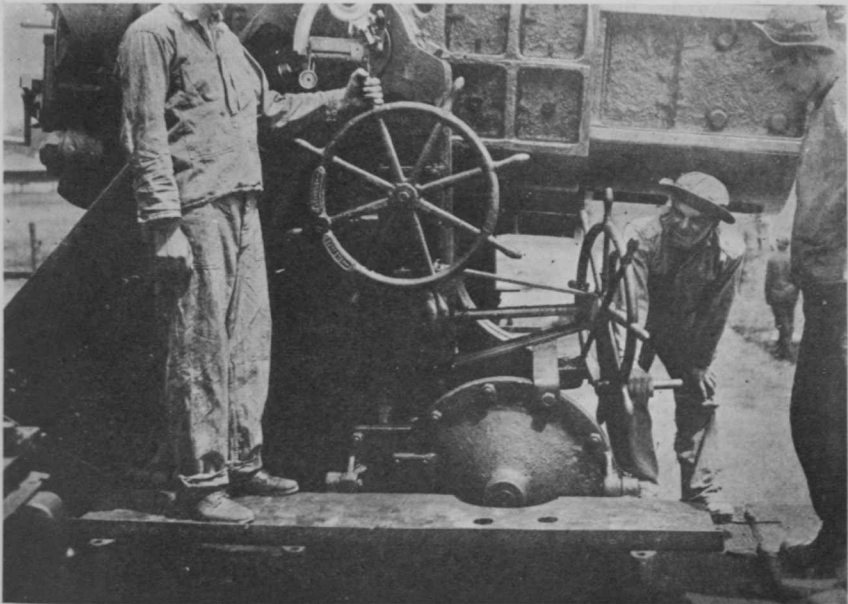
MODIFIED ELEVATION DEVICE FOR RAILWAY MORTARS
