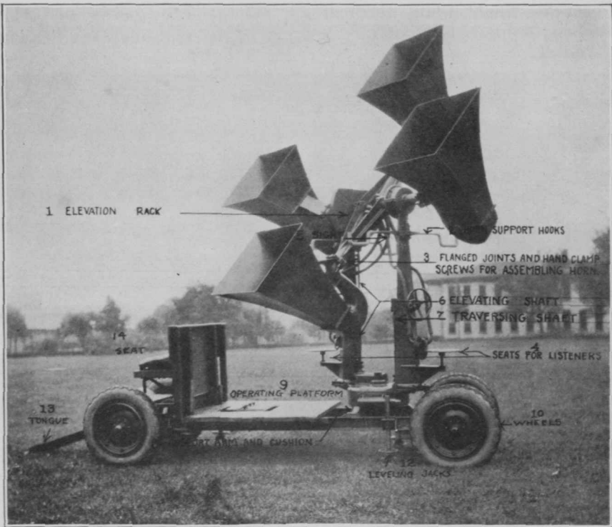
FIG. 9. SOUND LOCATOR
