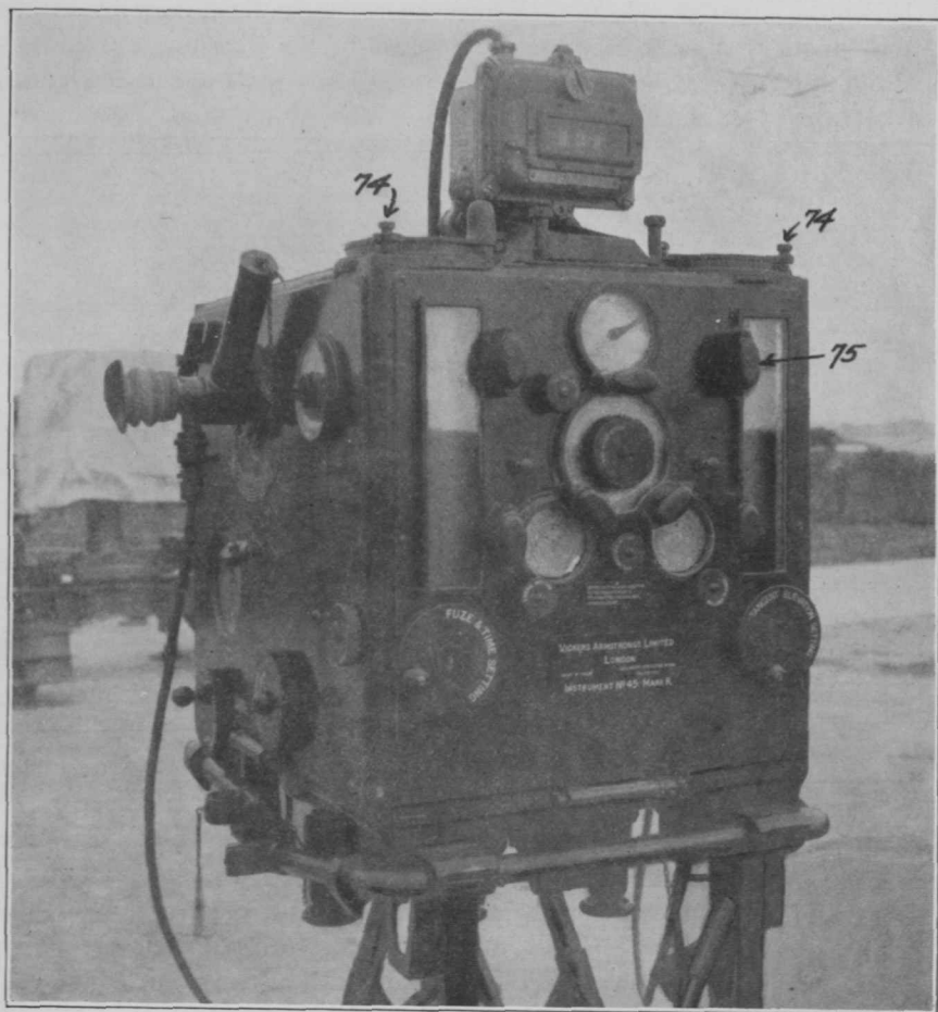
FIG. 5. DIRECTOR M-1 (VICKERS) No. 45
