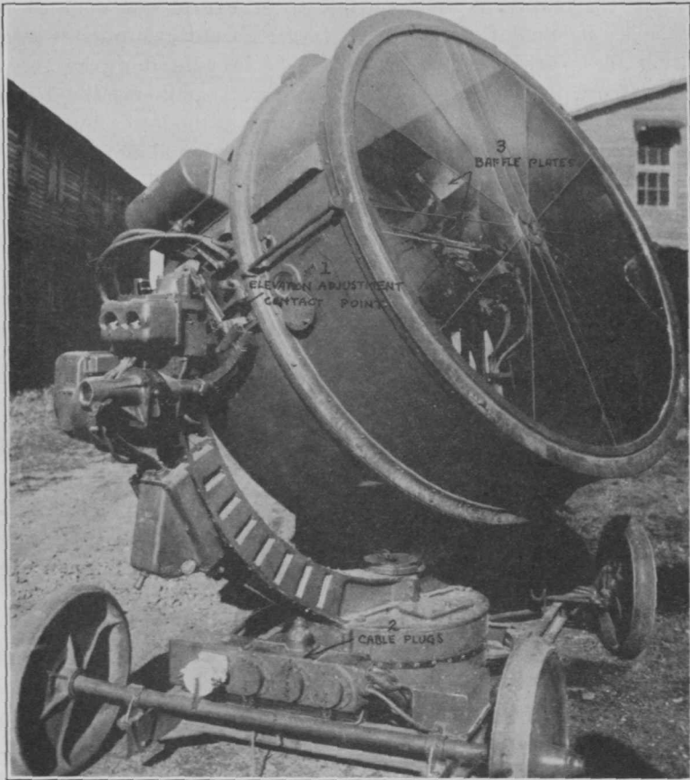
FIG. 8. SEARCHLIGHT
