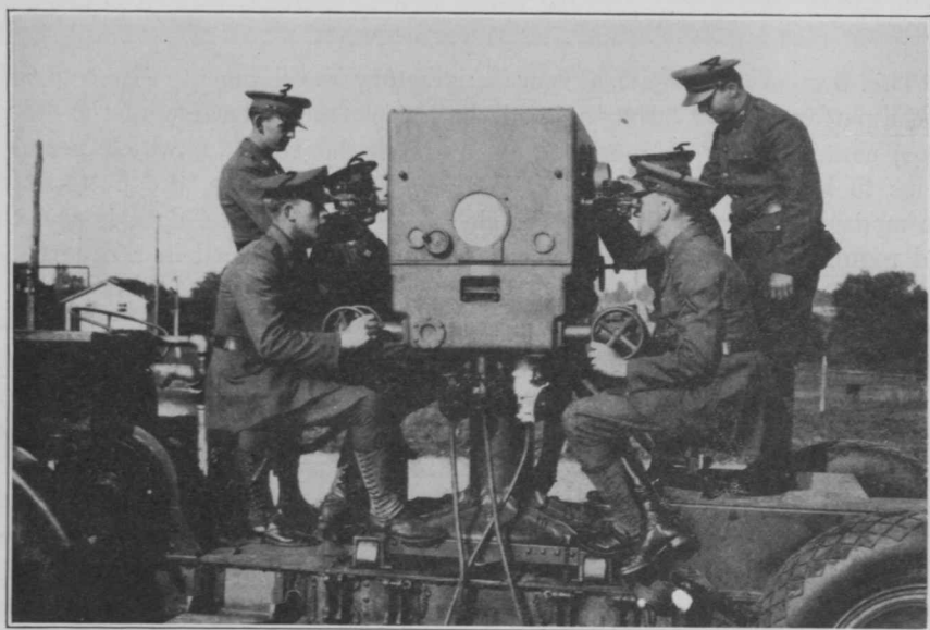
FIG. 7. DIRECTOR T-4
