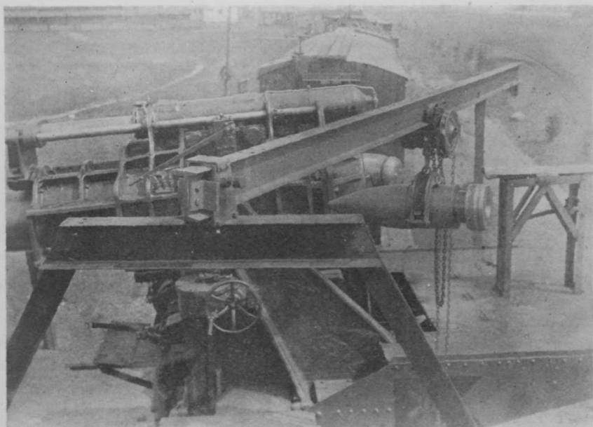
OVERHEAD LOADING DEVICE FOR RAILWAY MORTARS
