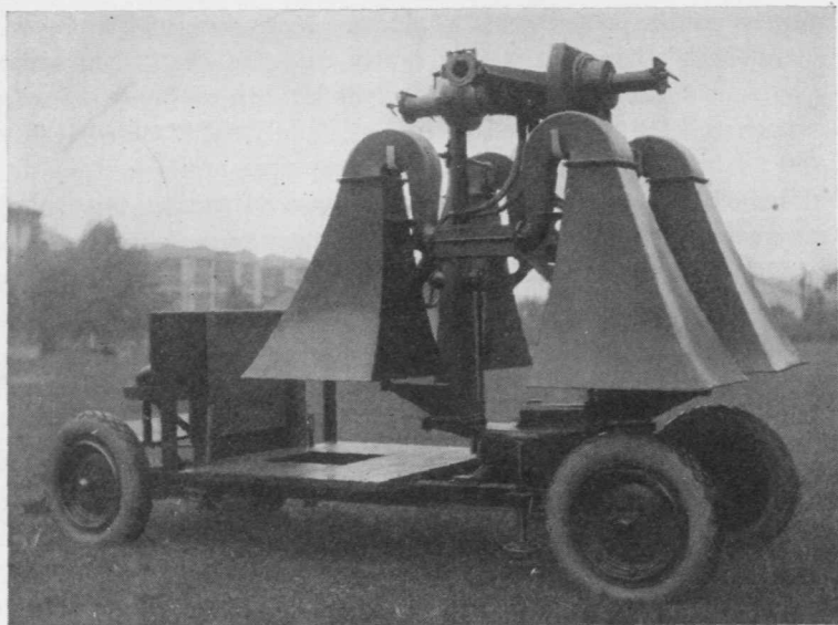
SOUND LOCATOR TRAILER WITH HORNS DISMOUNTED AND LOCKED IN TRAVELING POSITION
