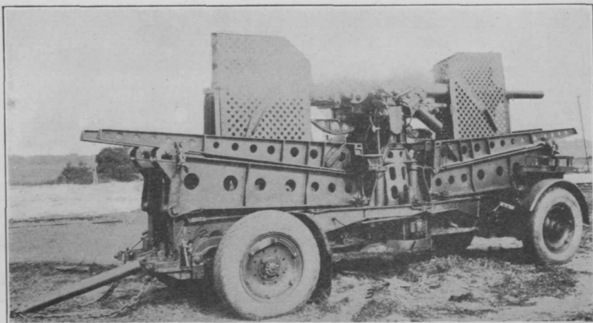
FIG. 2. 3-INCH ANTI-AIRCRAFT GUN IN TRAVELING POSITION
