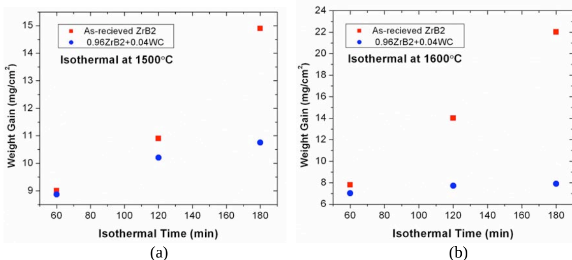
Figure 4. Normalized mass gain as a function of time for nominally pure \text{ZrB}_2 (squares) and (\text{Zr,W})\text{B}_2 (circles) oxidized in flowing air (a) 1500°C and (b) 1600°C. Note the difference in Y-axis scales for the two plots.
