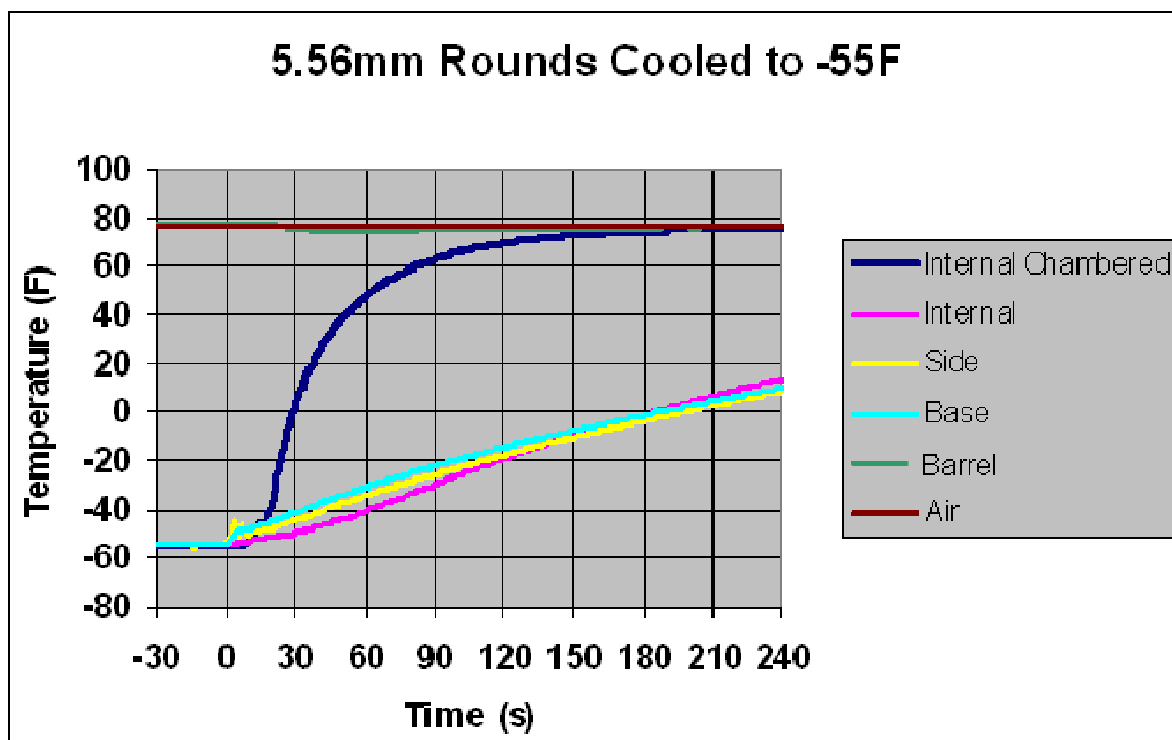
Figure 15. Time to warm single 5.56mm cartridges from -55 °F to ambient.
