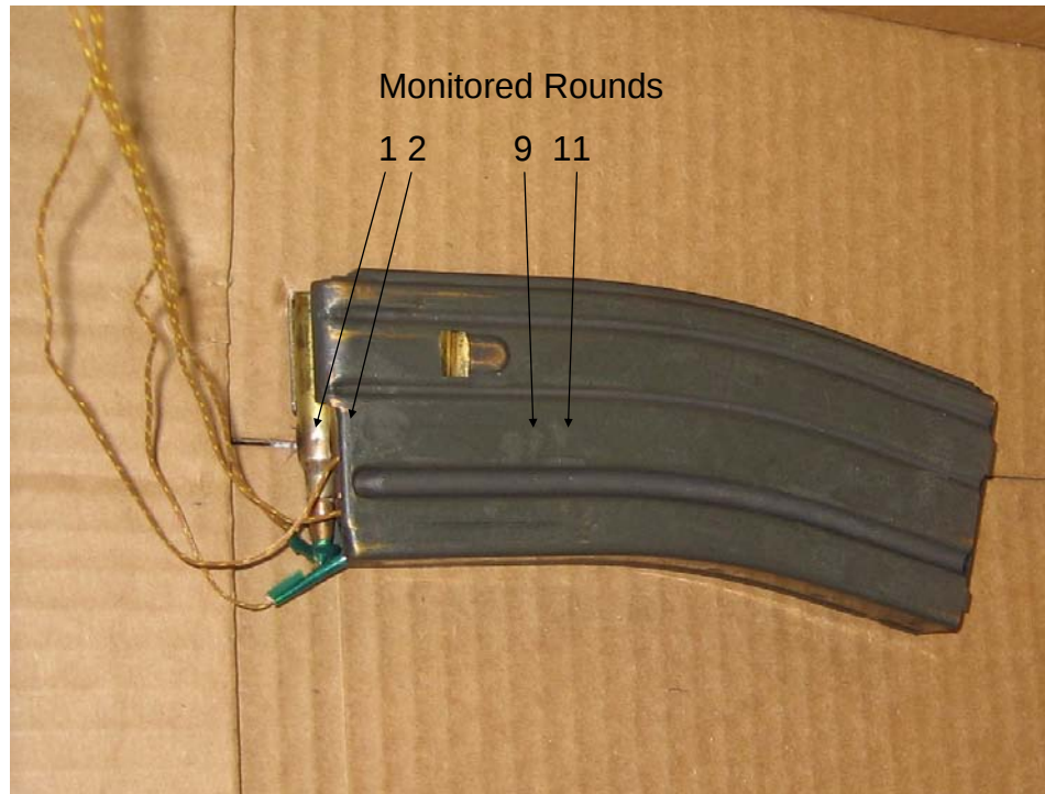
Figure 5. The 30 round magazine loaded with thermal coupled cartridges.
