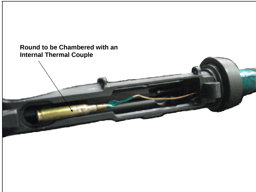
Figure 4. The 5.56mm cartridge with internal thermal couple for chambering into M4 barrel.
