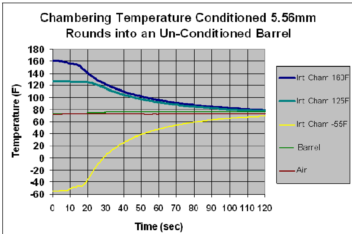
Figure 16. The effect of chambering temperature-conditioned 5.56mm cartridges into an unconditioned barrel.
