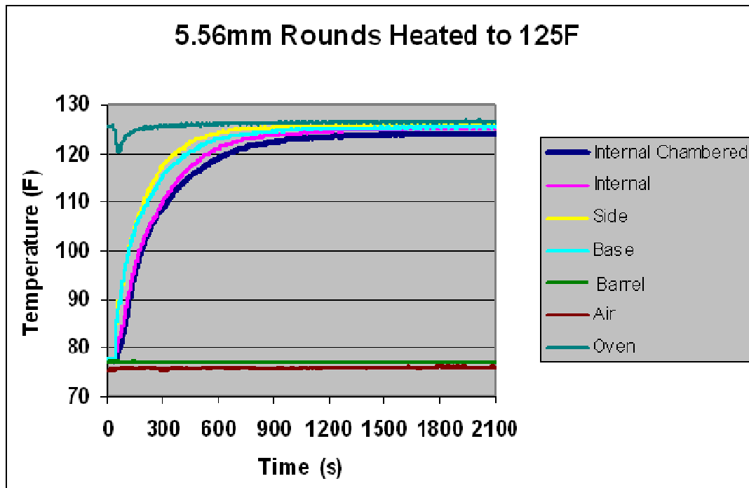
Figure 7. Time to condition single 5.56mm cartridges to 125 °F.
