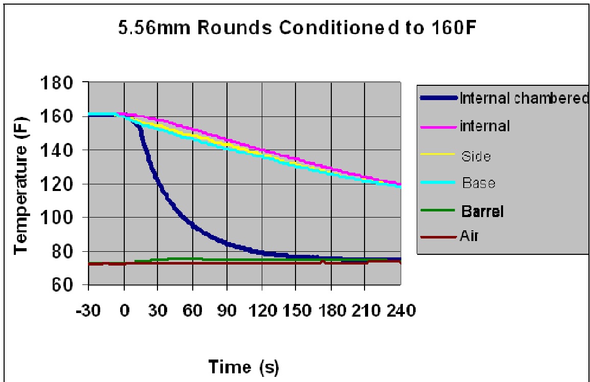
Figure 13. Time to cool single 5.56mm cartridges from 160 °F to ambient.
