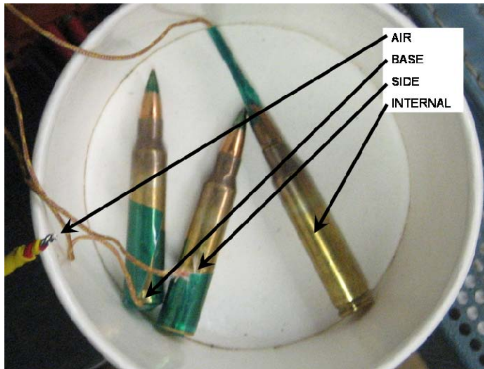
Figure 1. The 5.56mm cartridges instrumented with thermal couples.
