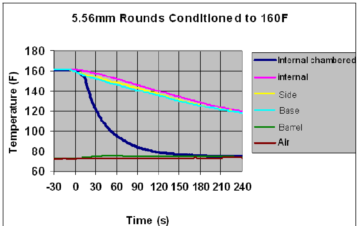
Figure 14. Time to cool single 5.56mm cartridges from 125 °F to ambient.
