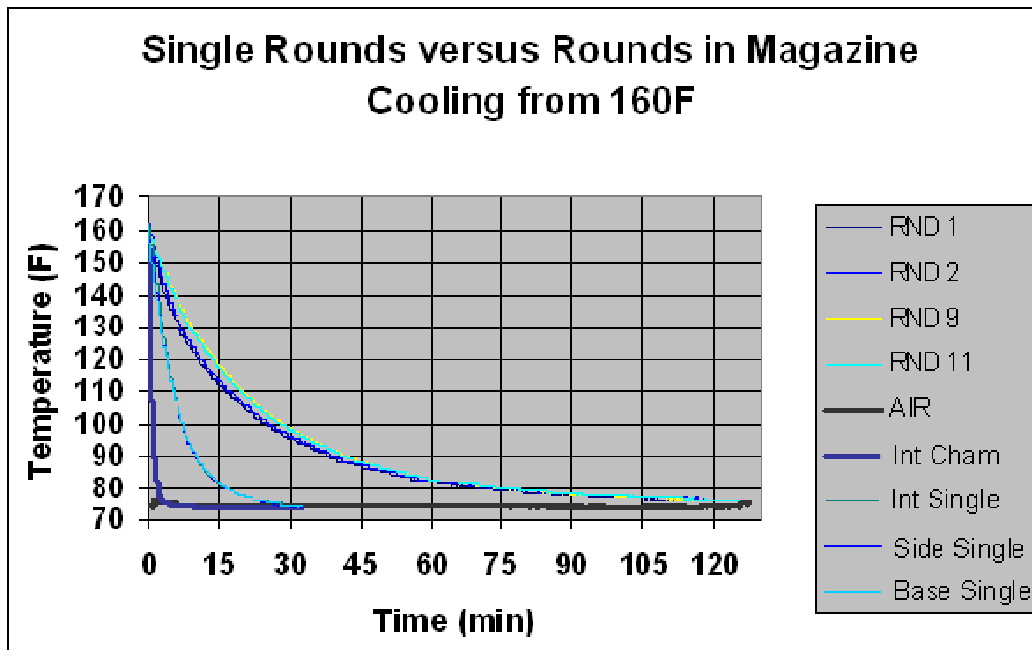
Figure 11. The return of rounds conditioning to 160 °F loaded into a magazine and single rounds to ambient temperature.
