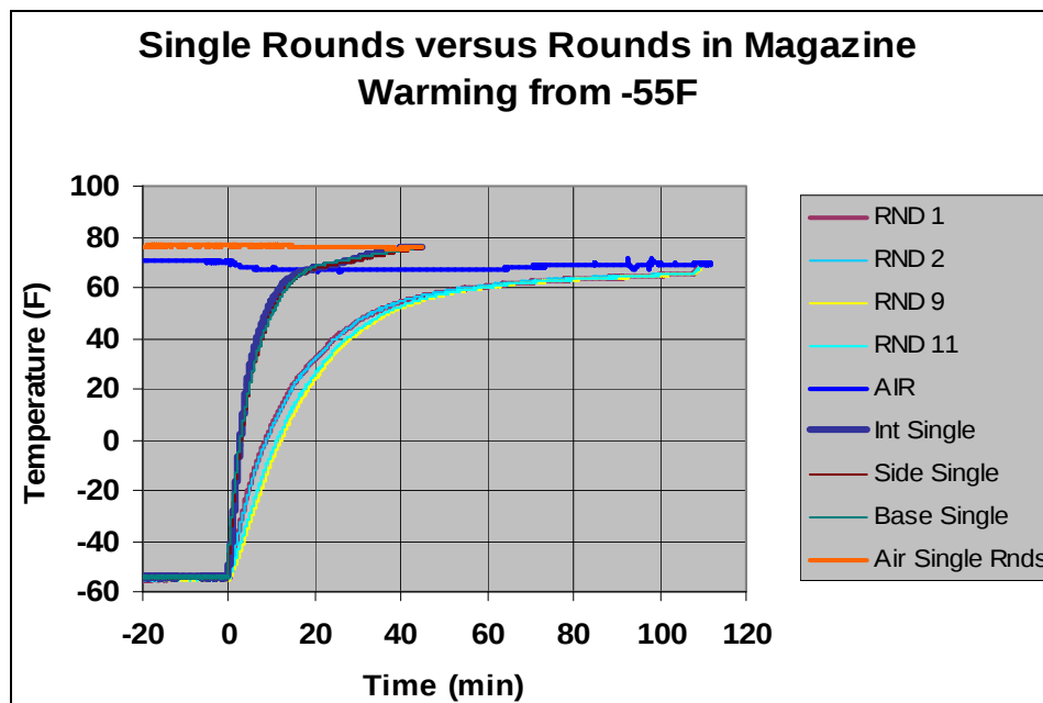
Figure 12. Time to return rounds loaded into a magazine and single rounds conditioned to -55 °F to ambient temperature.
