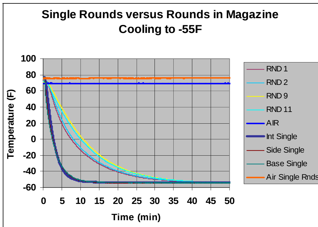
Figure 10. Time to condition rounds loaded into a magazine and single rounds to -55 °F.
