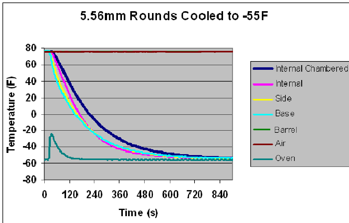
Figure 8. Time to condition single 5.56mm cartridges to -55 °F.
