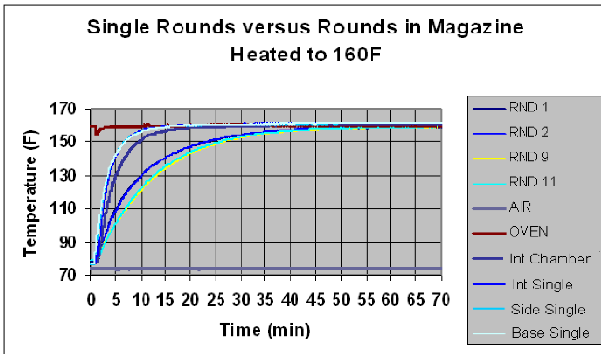
Figure 9. Conditioning to 160 °F of rounds loaded into a magazine and single rounds.
