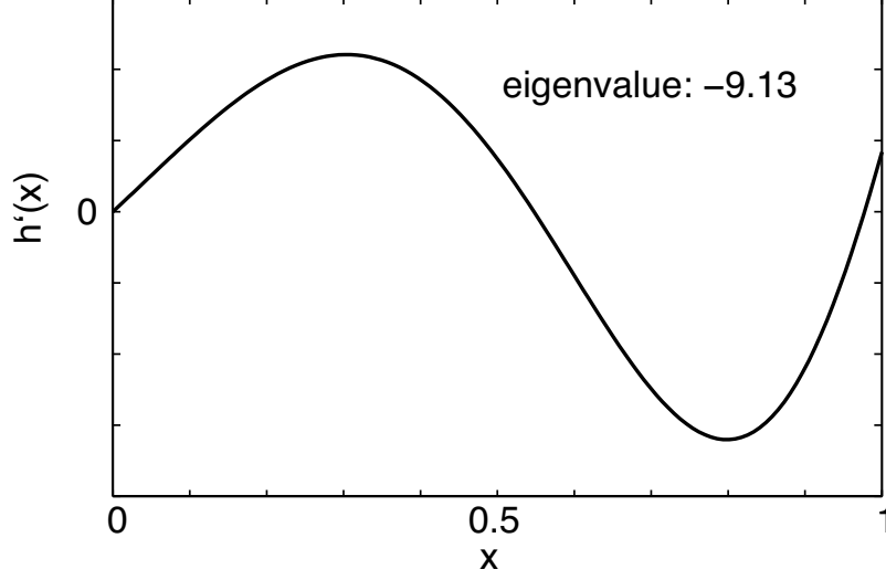
Figure 3: An eigenfunction of the dispersion function of eq. (64). Solutions correspond to decaying modes only, with negative real part eigenvalues.
