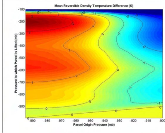
Figure 9: Contour plot of the difference between the environmental density temperature and the density temperature of a parcel lifted reversibly and adiabatically from the pressure level given on the abscissa to the pressure level on the ordinate. This quantity has been averaged over several thousand soundings taken at Kapingamarangi in the tropical western South Pacific.
