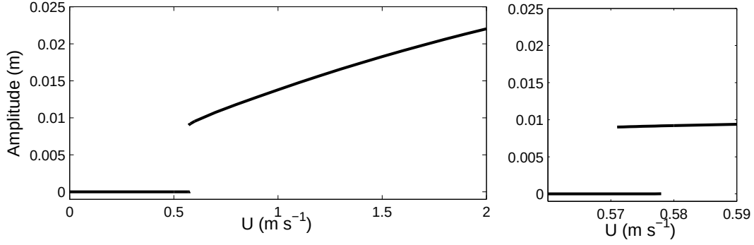
Figure 17: Bifurcation diagram for shallow water model showing oscillation amplitudes as a function of water speed. On the right is an enlarged view of the transition. The steady state becomes linearly unstable at around 0.578 and the upper (bouncing) branch loses stability at around 0.571. m = 3.4 g, \mu = 0.2 kg s -1 and \lambda = 1 .
