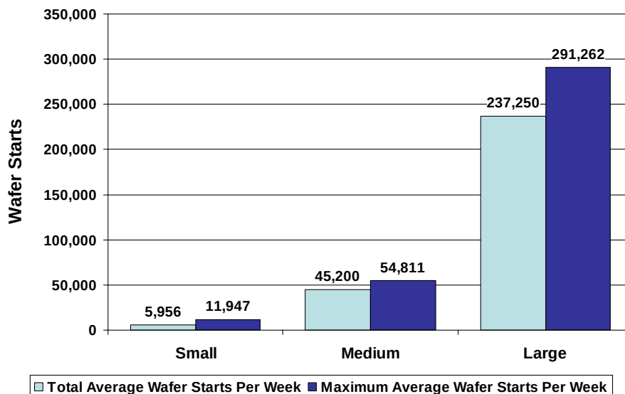
Figure VII-3: Wafer Starts per Week (2007)
