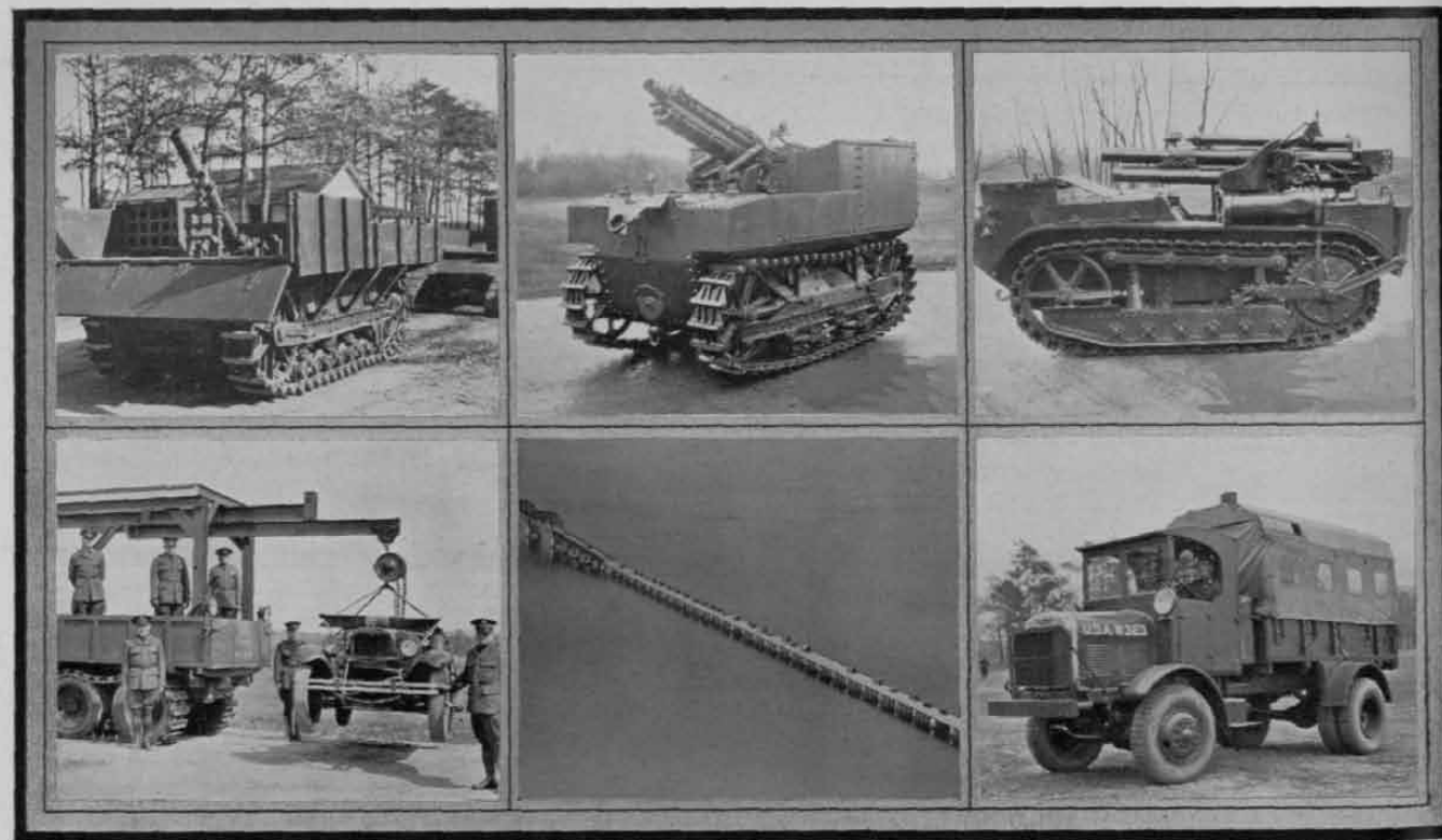
Top Row Left to Right—The 4.2-inch Chemical Mortar on a T1E1 Chassis; 75-mm. Pack Howitzer Motor Carriage, T1; American 75-mm. Gun on Mark VII Self-propelled Mount.
