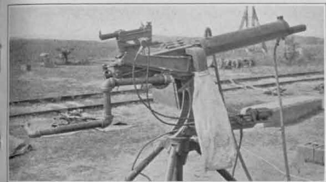
Cal. .50 Antiaircraft M. G. with Back Rest Installed
