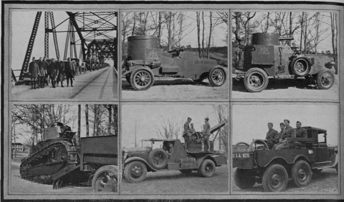
Top Row Left to Right—Mechanized Force Crossing James River Bridge, January 27, 1931; Light Armored Car Equipped with one Caliber-.30 Air-cooled Browning M. G. Weight 4142 Pounds; Franklin Medium Armored Car, Equipped with one Caliber-.50 and two Caliber-.30 Browning Air-cooled M. G.'s. Weight, 7138 Pounds.
