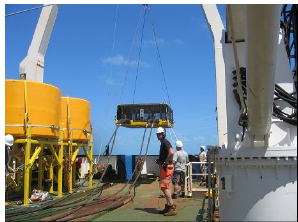
Figure 17 J-Box Deployment
