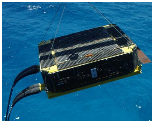
Figure 2 STAFAC J-Box
