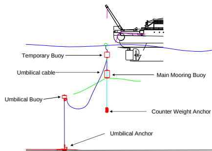
Figure 36 Umbilical Cable Shackled to Temporary Array Cable
