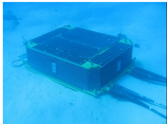
Figure 18 J-Box Lowered to the Seafloor
