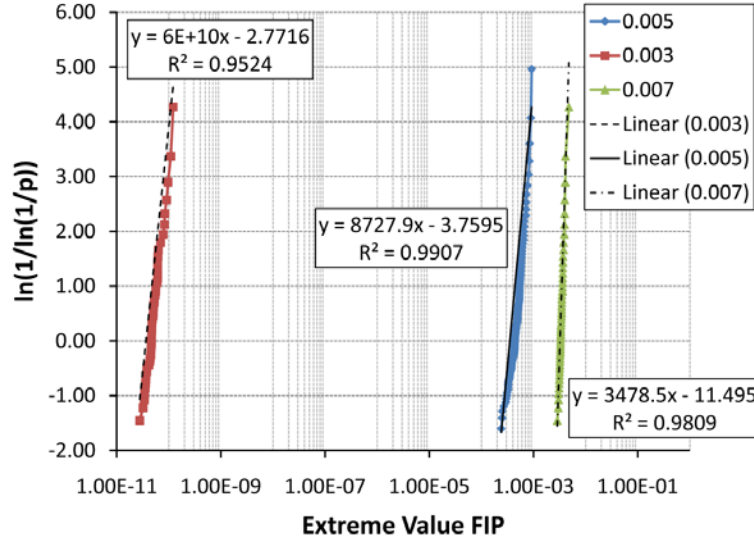
Figure 10 The extreme value distribution of the Fatemi-Socie FIP as estimated over a single element and over the entire grain for the simulations cycled at 0.3%, 0.5%, and 0.7% strain. The extreme value Fatemi-Socie FIP was selected to be the FIP with the highest magnitude out of all the FIP calculated over each element or over each grain in each SVE.
