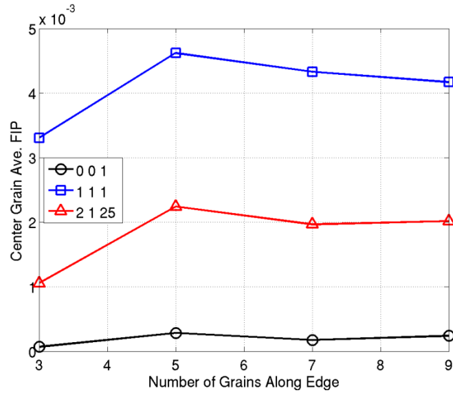
Figure 7 Comparison of the grain averaged Fatemi-Socie FIP of the center grain oriented with its {0 0 1}, {1 1 1} and {2 1 25} planes perpendicular to the loading directions, respectively, versus the number grains along the edge of the SVE. These SVEs consisted of arrays of cuboidal grains each grain dimensioned 9\mu\text{m} along an edge.
