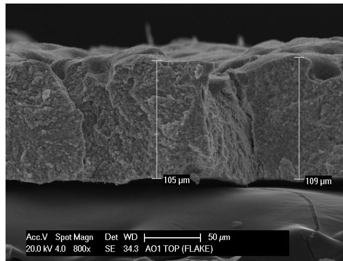
Figure 4: Approximate cross-sectional thickness of a single layer thermal barrier coating (100% ceramic).
