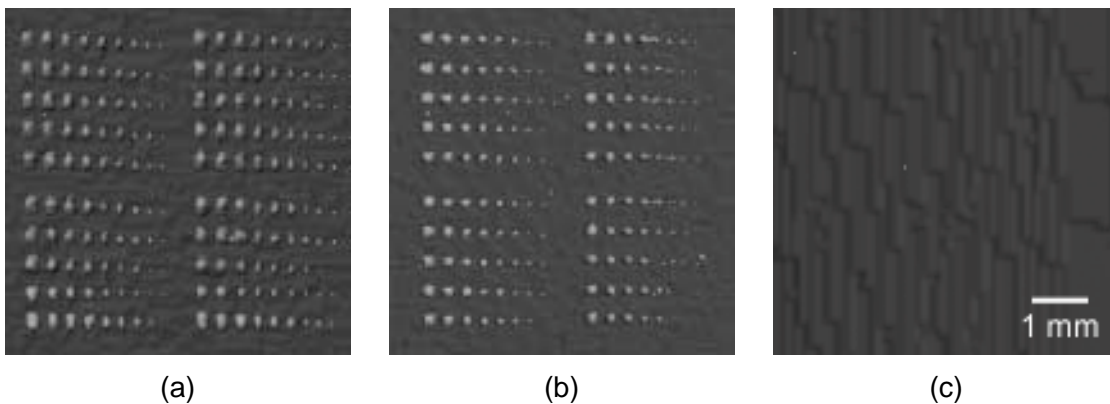
Fig. 6. Reconstructed polychromatic micro-CT images at 10 μm resolution for gold islands deposited to a thickness of (a) 1 μm, (b) 500 nm and (c) 100 nm.
