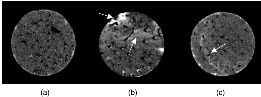
Fig. 14. Specimen cross-sections (2.5 mm diameter) imaged by micro-CT showing (a) non-specific BaSO 4 staining (bright voxels) in unloaded control specimens, and (b,c) regions of concentrated BaSO 4 staining in specimens loaded in cyclic uniaxial tension. Arrows highlight regions of BaSO 4 staining characteristic of fatigue damage and/or propagating microcracks.
