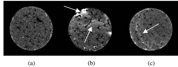
Fig. 1. Specimen cross-sections (2.5 mm diameter) imaged by micro-CT showing (a) non-specific BaSO 4 staining (bright voxels) in unloaded control specimens, and (b,c) regions of concentrated BaSO 4 staining in specimens loaded in cyclic uniaxial tension. Arrows highlight regions of BaSO 4 staining characteristic of fatigue damage and/or propagating microcracks.
