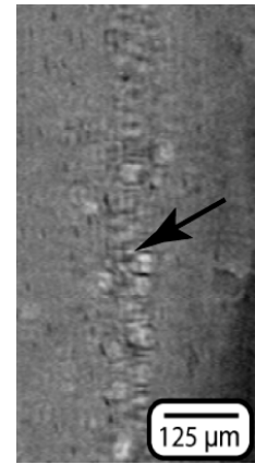
Fig. 7. Synchrotron x-ray tomography slice of bovine cortical bone specimen showing enhanced contrast in the scratched region (labeled by an arrow) corresponding to the presence of alendronate functionalized Au NPs.
