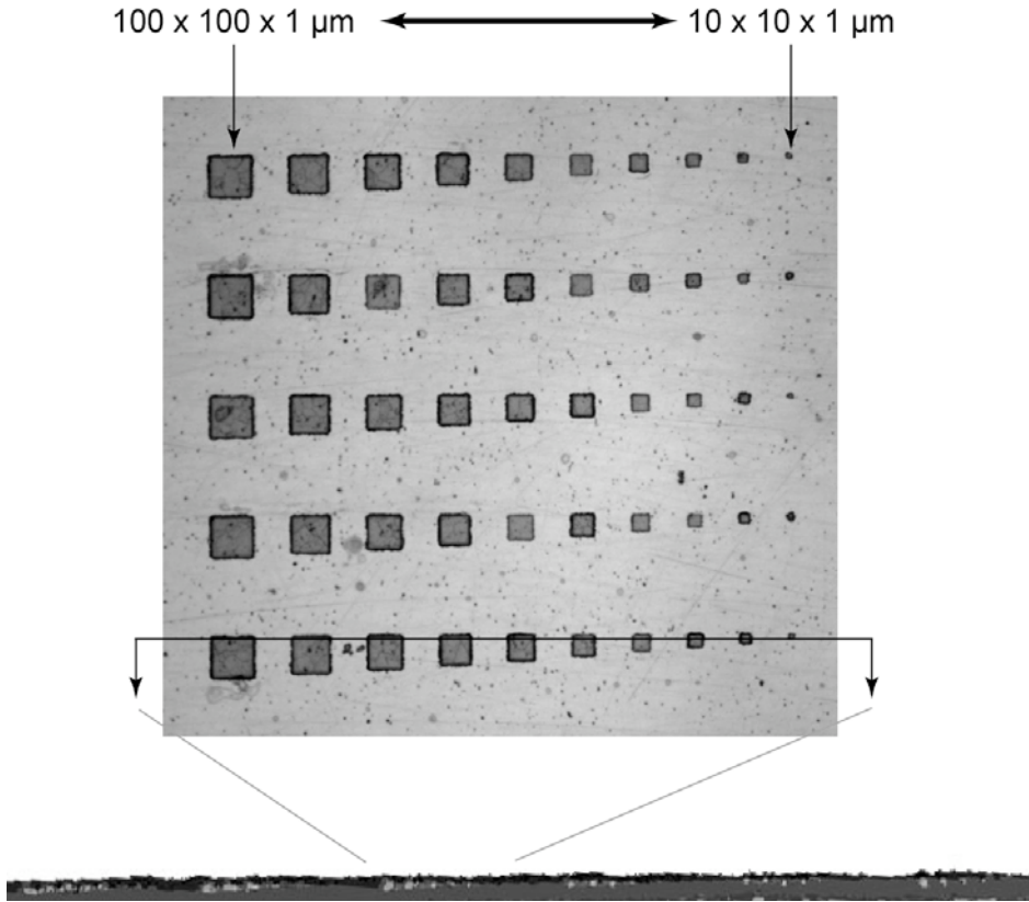
Fig. 5. Optical micrograph (above) showing an array of gold islands (darker) deposited on an aluminum (lighter) substrate and a thresholded micro-CT slice (below) at 10 μm resolution showing the gold islands (brighter) in cross-section on the surface of the aluminum (darker) substrate.
