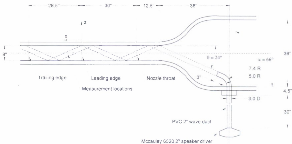
Figure 1. Speaker driver with 66° wave duct.
