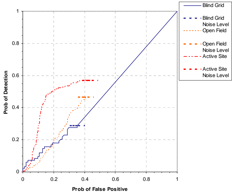
Figure 6. GEM-5/TOWED ARRAY P_d^{\text{res}} stages versus the respective P_{\text{fp}} over all ordnance categories combined.
