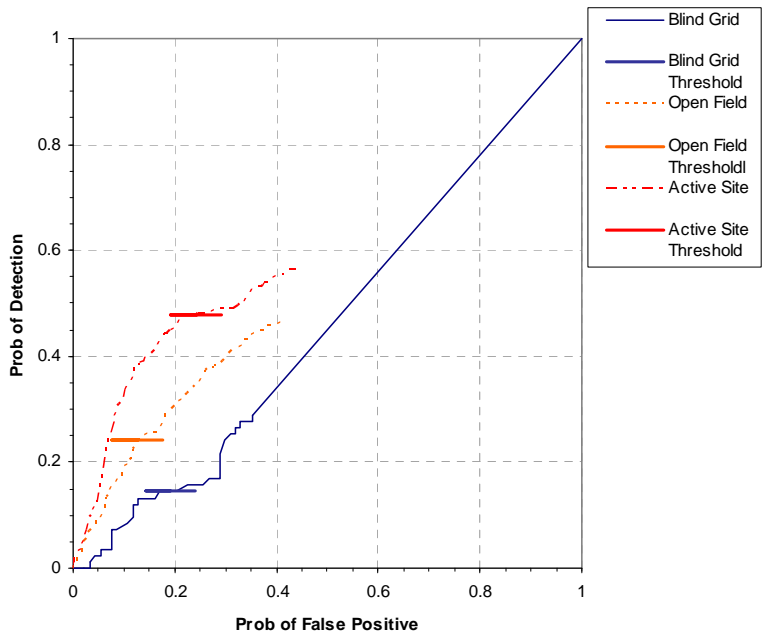
Figure 7. GEM-5/TOWED ARRAY P_d^{\text{disc}} versus the respective P_{\text{fp}} over all ordnance categories combined.
