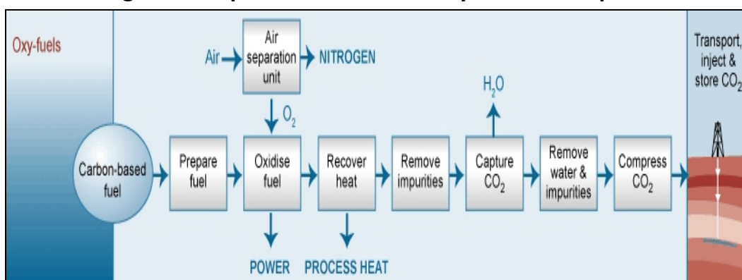
Figure 3. Simplified Illustration of Oxy-Fuel CO 2 Capture
