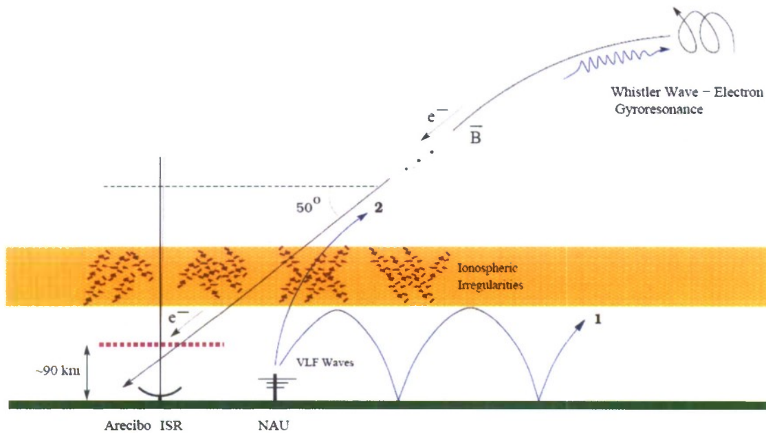
Figure 2. Geometry and scenario of Arecibo experiments. Signals at 40.75 kHz emitted from NAU can propagate either as subionospheric waves (denoted by Ray 1) or whistler-mode waves along the Earth's magnetic field in the ionosphere (denoted by Ray 2). The coupling of NAU signals into the ionosphere is enhanced by ionospheric irregularities. Whistler-mode waves can then interact with energetic electrons in radiation belts at L = 1.35 , and subsequently cause electron precipitation into the lower ionosphere over Arecibo.
