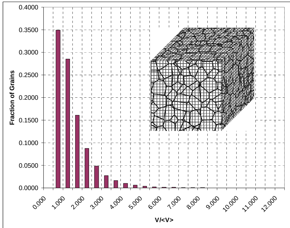
Figure 6. Log normal distribution of grain volume V normalized by imposed average grain volume \langle V \rangle of 1 \times 10^{-5} \text{ mm}^3 which corresponds to a cube root grain size of 20 \mu\text{m} .
