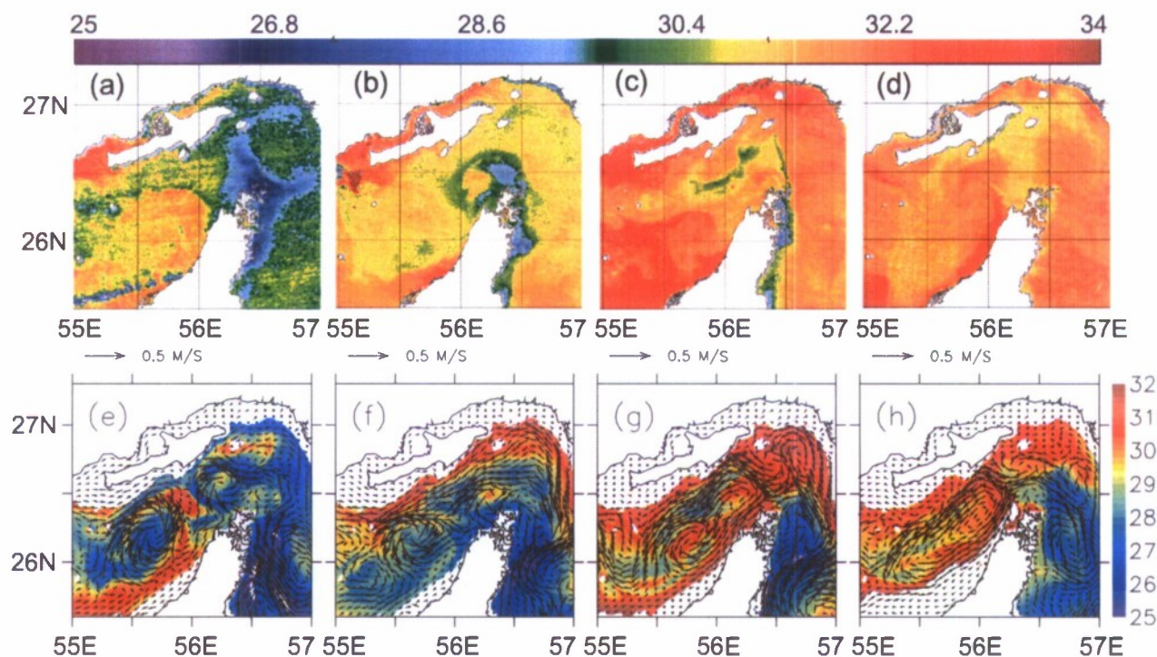
FIG. 9. MODIS ( \sim 1 km) SST imagery during (a) 12 Jul and (b) 20 Jul, (c) 25 Aug, and (d) 26 Sep 2005 and (e)–(h) model temperatures at 20 m with overlaid currents in the upper 40 m for the same period. Model temperature at 20 m is shown because the eddy has a weaker signature at the surface than at the subsurface owing to the strong near-surface stratification.
