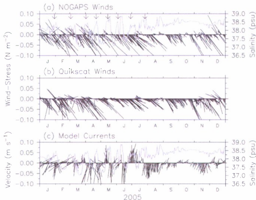
FIG. 14. (a) Stick plot of \frac{1}{2}^{\circ} NOGAPS wind stress averaged for the Persian Gulf region (west of 56^{\circ}\text{E} ) and model salinity at 40 m ( 26.26^{\circ}\text{N} , 56.08^{\circ}\text{E} , gray line) in the Strait of Hormuz during 2005. (b) Stick plot of QuikSCAT wind stress, which is included for comparison. (c) Volume-averaged ( 26^{\circ} – 27^{\circ}\text{N} , 55.9^{\circ} – 56.4^{\circ}\text{E} , 0–100 m) simulated currents ( \text{m s}^{-1} ) and salinity at 40 m at 26.26^{\circ}\text{N} , 56.08^{\circ}\text{E} . The 3-hourly, \frac{1}{2}^{\circ} NOGAPS wind stress is interpolated to a daily \frac{1}{4}^{\circ} QuikSCAT grid before averaging. A constant drag coefficient ( C_D ) value of 1.2 \times 10^{-3} is used to compute the wind stress from the QuikSCAT wind velocity. A daily QuikSCAT wind stress has been generated by taking 3-day moving averages. Eight dominant salinity events are marked by arrows.
