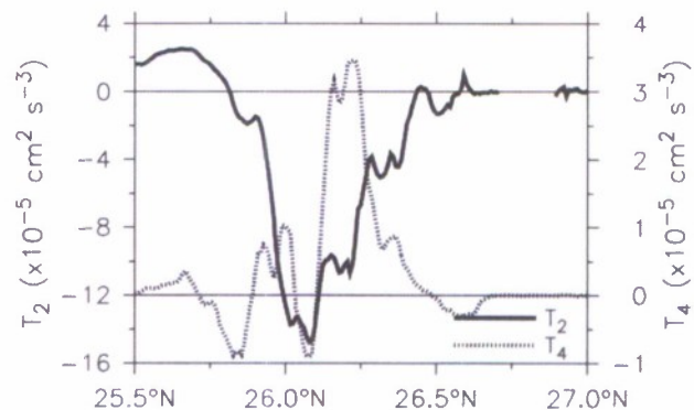
FIG. 17. Latitudinal dependence of the eddy-mean flow interaction terms involving baroclinic ( T_2 ) and barotropic ( T_4 ) instability between 55° and 56°E for the upper 100 m during June 2005. The T_2 and T_4 terms are calculated using the Eqs. (14) and (16) from Böning and Budich (1992), respectively.
