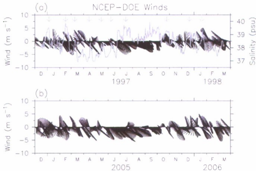
FIG. 13. (a) Stick plot of NCEP-DOE reanalysis wind velocity vectors averaged over the Persian Gulf region (west of 56°E) and the observed salinity at 40 m in the Strait of Hormuz [26.26°N, 56.08°E; Johns et al. (2003)] during December 1996–March 1998 (gray line). Salinity is sampled at 30 s and winds are available for 6-h intervals. A 2-day Parzen smoothing is applied to the salinity to highlight the episodic variations in the high-salinity outflow. Arrows mark periods of increased salinity outflow events. (b) The same wind vectors as in (a) but for the period 2004–06.
