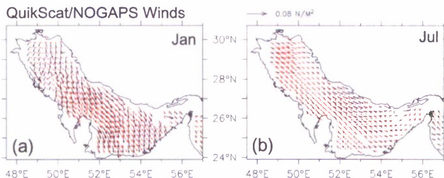
FIG. 2. A comparison of wind stress derived from the QuikSCAT (black vectors) and NOGAPS (red vectors) for (a) January 2005 and (b) July 2005 in \text{N m}^{-2} . The 3-hourly, \frac{1}{2}^\circ NOGAPS wind stress is interpolated to a daily \frac{1}{4}^\circ QuikSCAT grid. A constant drag coefficient ( C_D ) value of 1.2 \times 10^{-3} is used to compute the wind stress from the QuikSCAT wind velocity. A daily QuikSCAT wind stress has been generated by taking 3-day moving averages.
