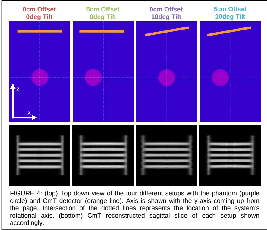
Figure 4 shows the four different CmT setups: (1) phantom at the center-of-rotation (COR) and no detector misalignment; (2) phantom 5cm offset from the COR and no detector misalignment; (3) phantom at the COR and detector tilted 10° respect to the y-axis; and (4) phantom 5cm offset from the COR and detector tilted 10° respect to the y-axis. Final reconstructed images showed that in an ideal situation with no detector tilt, there was no visible cylindrical artifact irrespective of offset. However with a detector tilt, a cylindrical artifact was only seen in the offset geometry. This was similar to what was seen with the actual reconstructed images collected with a Defrise phantom on the built system (Fig. 2). A line profile taken through the center of the middle (3 rd from top) disc confirms the cylindrical artifact seen in the 5cm offset and 10° tilt case with the sudden noticeable
