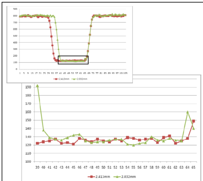
FIGURE 6 (top) Line profile across a single lead shot with diameters of 2.032 and 2.413mm. (bottom) Enlarged view of the profile marked by the black box.
