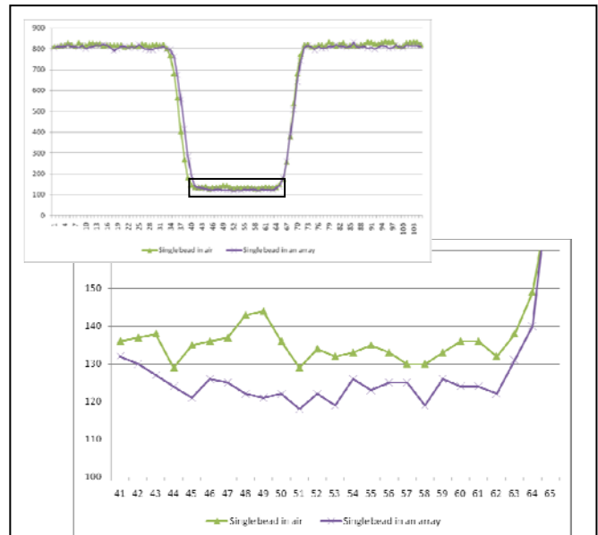
FIGURE 7 (top) Line profile across a single lead bead in air and in an array with multiple beads. (bottom) Enlarged view of the profile marked by the black box.
