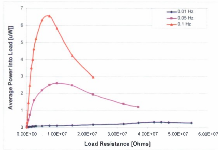
Figure 4.19. Average power at the electrical load for small frequency conditions with respect to load resistance
