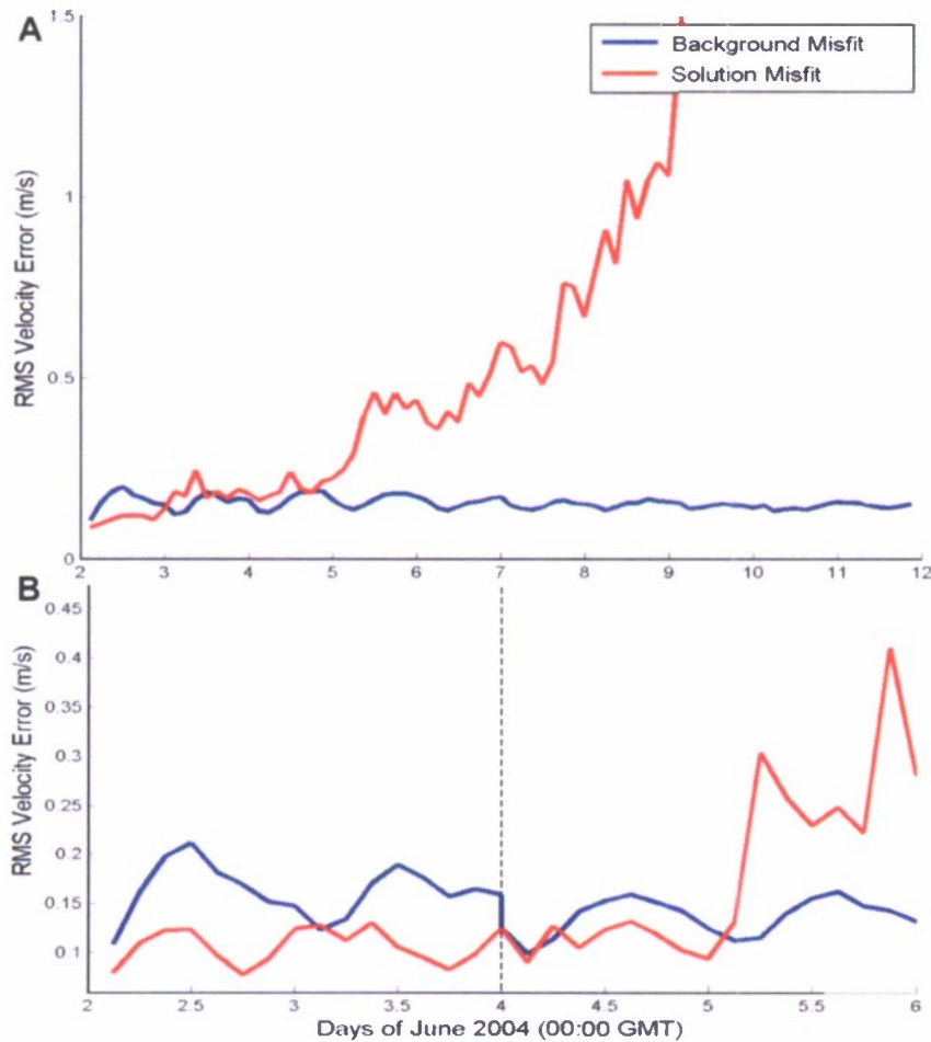
Fig. 6. \text{RMS}(\{L[u] - d\}) is computed and plotted at each 3-h data sampling time stamp. L is the measurement functional that projects the velocity field from state space to data space, d is the data, and u represents velocity from the nonlinear background (blue) and the assimilated solution (red). (A) Ten day assimilation experiment. (B) Two day cycling experiment, where the dashed line represents the break between cycles.
