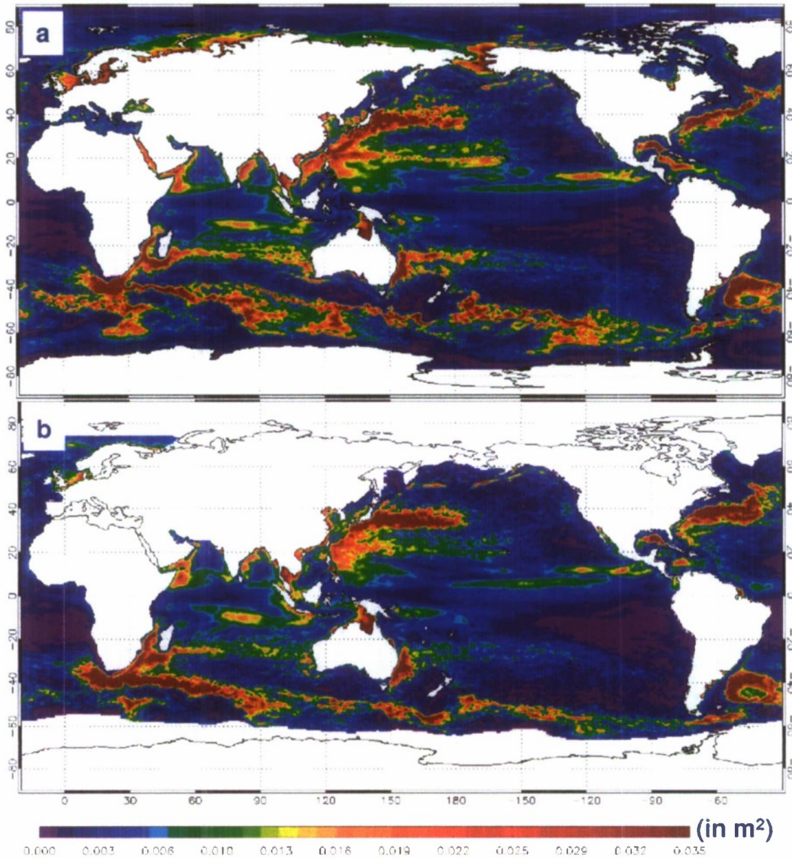
Figure 1: 2004-2006 Sea Surface Height (SSH) variability ( \text{m}^2 ) calculated (a) from the 1/12^\circ global Mercator Océan configuration, ORCA12, run without ocean data assimilation and (b) from satellite altimeter data.
