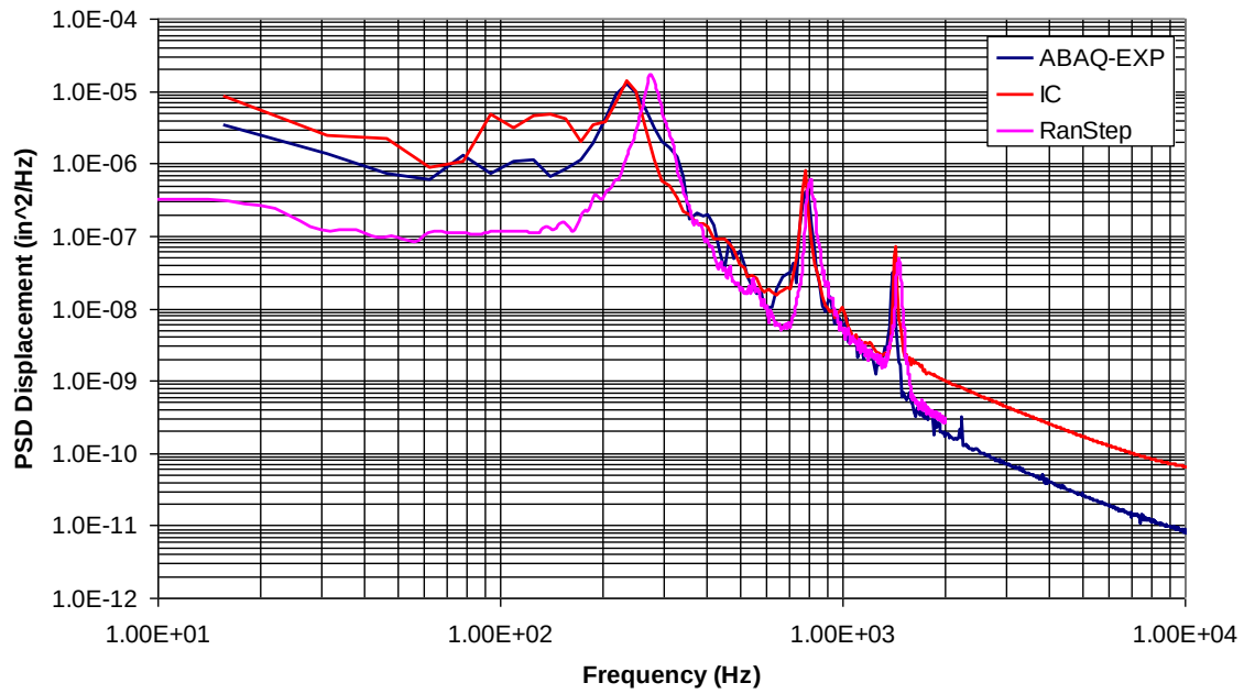
Figure 31 – Vertical Displacement, Prms=0.92psi, 3-Modes, Alpha=64., T=2secs
