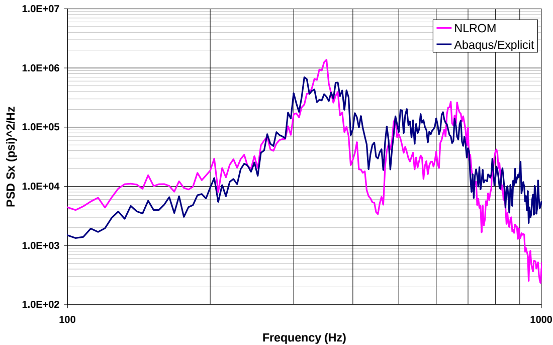
Figure 78 – Stress in the Clip at the Edge of Panel, OASPL = 165 dB, Ps=3psi
