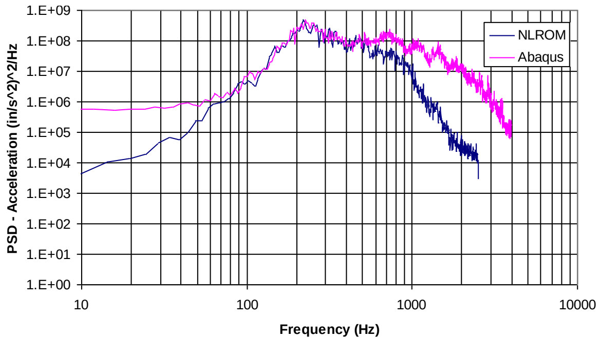
Figure 40 – Out-of-Plane Z-Acceleration at the Center of the Panel
