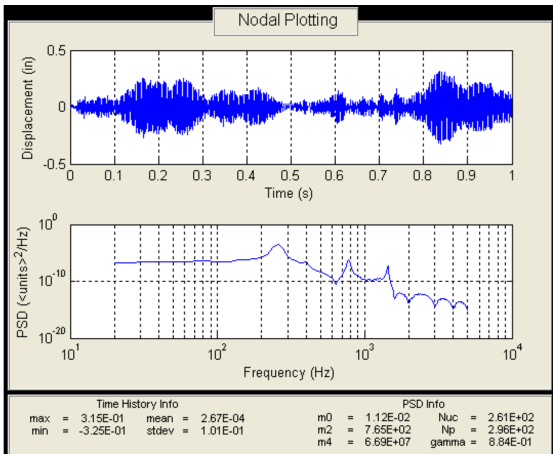
Figure 19 – Nodal Post-Processing
