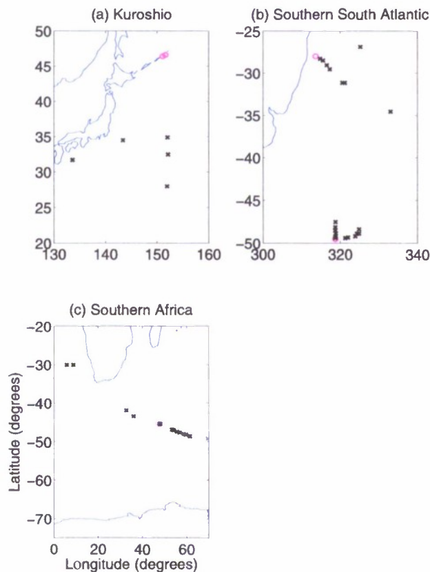
Figure 10. As in Figure 6, but for three subregions outside of the North Atlantic domain. (a) Kuroshio ( M=8 , \overline{D}_{\text{average}}=12 ). (b) Southern South Atlantic ( M=22 , \overline{D}_{\text{average}}=22 ). (c) Southern Africa ( M=13 , \overline{D}_{\text{average}}=3.5 ).
