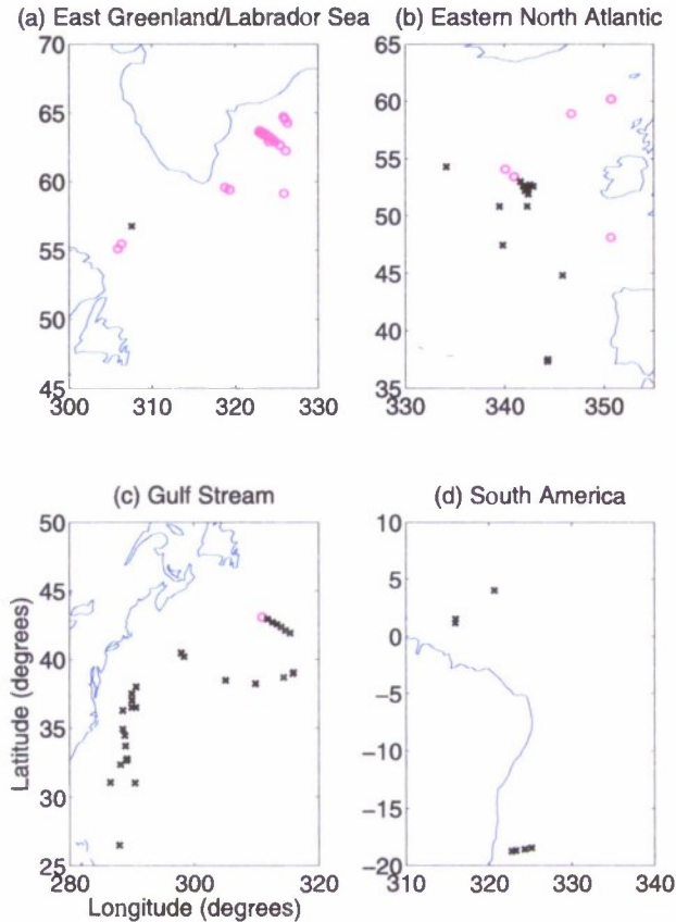
Figure 6. Current meters with large time-averaged currents (see text) in four subregions of the North Atlantic domain. Values of M (number of moorings) and \bar{D}_{average} = 0.0025 \rho |\mathbf{u}_b|^3 averaged over all of the moorings (units in \text{mW m}^{-2} ), are listed below. (a) East Greenland/Labrador Sea ( M = 35 , \bar{D}_{average} = 40 ). (b) Eastern North Atlantic ( M = 27 , \bar{D}_{average} = 8.9 ). (c) Gulf Stream ( M = 31 , \bar{D}_{average} = 6.7 ). (d) South America ( M = 7 , \bar{D}_{average} = 6.7 ). As in Figure 2, black crosses denote locations with seafloor depths exceeding 3000 m, and magenta circles denote locations with seafloor depths between 1000 and 3000 m.
