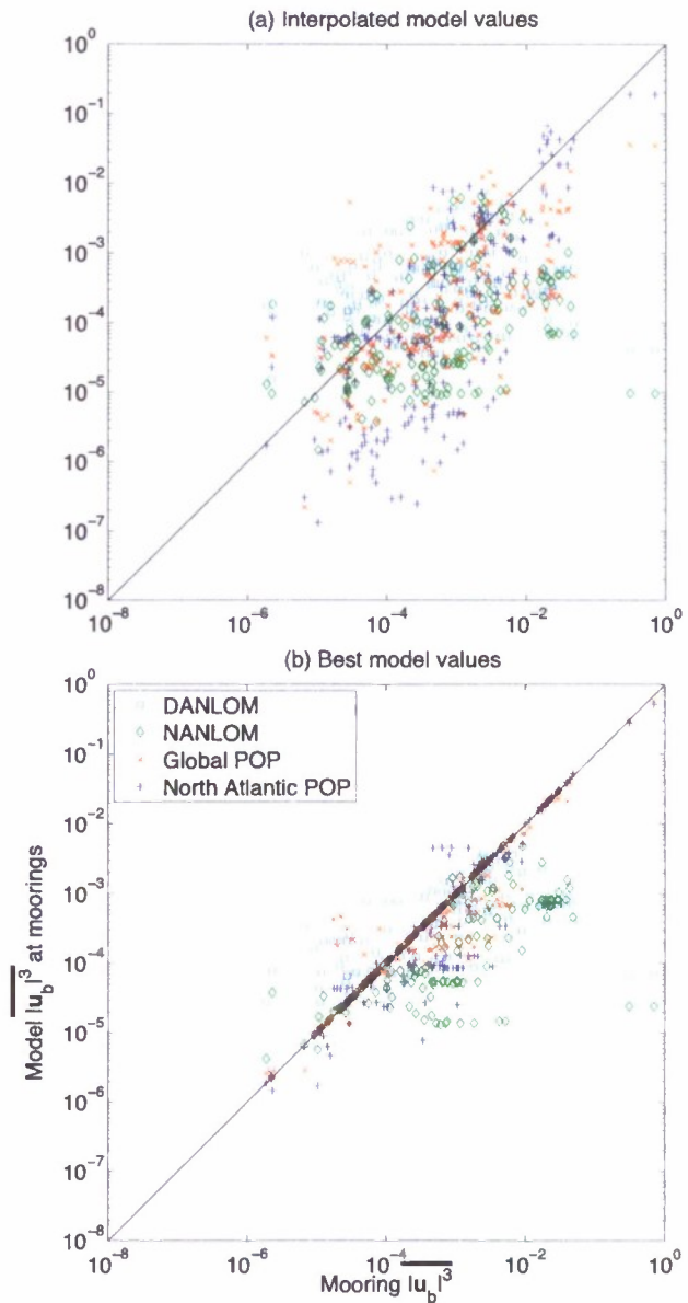
Figure 4. As in Figure 3 except that model |u_b|^3 values are plotted versus mooring |u_b|^3 values.
