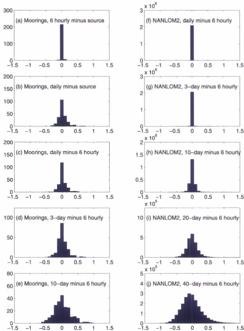
Figure 11. Histograms of \alpha = \frac{|u_b|_{I2}^3 - |u_b|_{I1}^3}{|u_b|_{I1}^3} , where I2 represents a coarser sampling interval and I1 represents a finer interval of the same data set. Results shown (a–e) for moored current meters and (f–j) for model grid points in NANLOM2 (a 6 hourly sampled nonassimilative simulation of NLOM). In Figures 11a, 11b, 11c, 11d, and 11e, source denotes the original mooring data, sampled at intervals from 15 min to 3 hours depending on the mooring. All other sampling intervals are given at the top of Figures 11a, 11b, 11c, 11d, 11e, 11f, 11g, 11h, 11i, and 11j. Only the 224 moorings and the 2094302 model grid points for which 0.0025 \rho |u_b|_{I1}^3 exceeds 1 \text{ mW m}^{-2} are used.
