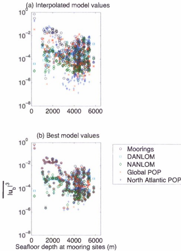
Figure 3. Values of |u_b|^3 computed from 187 moored near-bottom North Atlantic current meters, alongside values at the mooring locations from North Atlantic POP and the North Atlantic sectors of DANLOM, NANLOM, and global POP, plotted versus the seafloor depths of the moorings. (a) Model values interpolated to the mooring coordinates. (b) Model values, taken from 1^\circ by 1^\circ boxes centered on the moorings, which compare most closely to the mooring values. Units of |u_b|^3 are \text{m}^3 \text{s}^{-3} .
