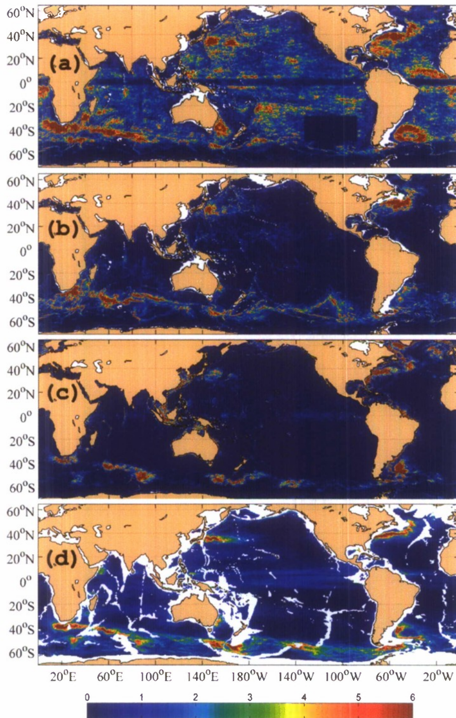
Figure 9. Maps of dissipation rate ( \text{mW m}^{-2} ) in the three global models (a) DANLOM, (b) NANLOM, and (c) global POP, and (d) in the [\bar{D}_3] observationally based estimate of Sen et al. [2008]. Figures 9a, 9b, 9c, and 9d extend to 65°N. A common value of c_d = 0.0025 was used to make Figures 9a, 9b, 9c, and 9d. Note that the Sen et al. [2008] estimate shown here only covers seafloor depths exceeding 3000 m.
