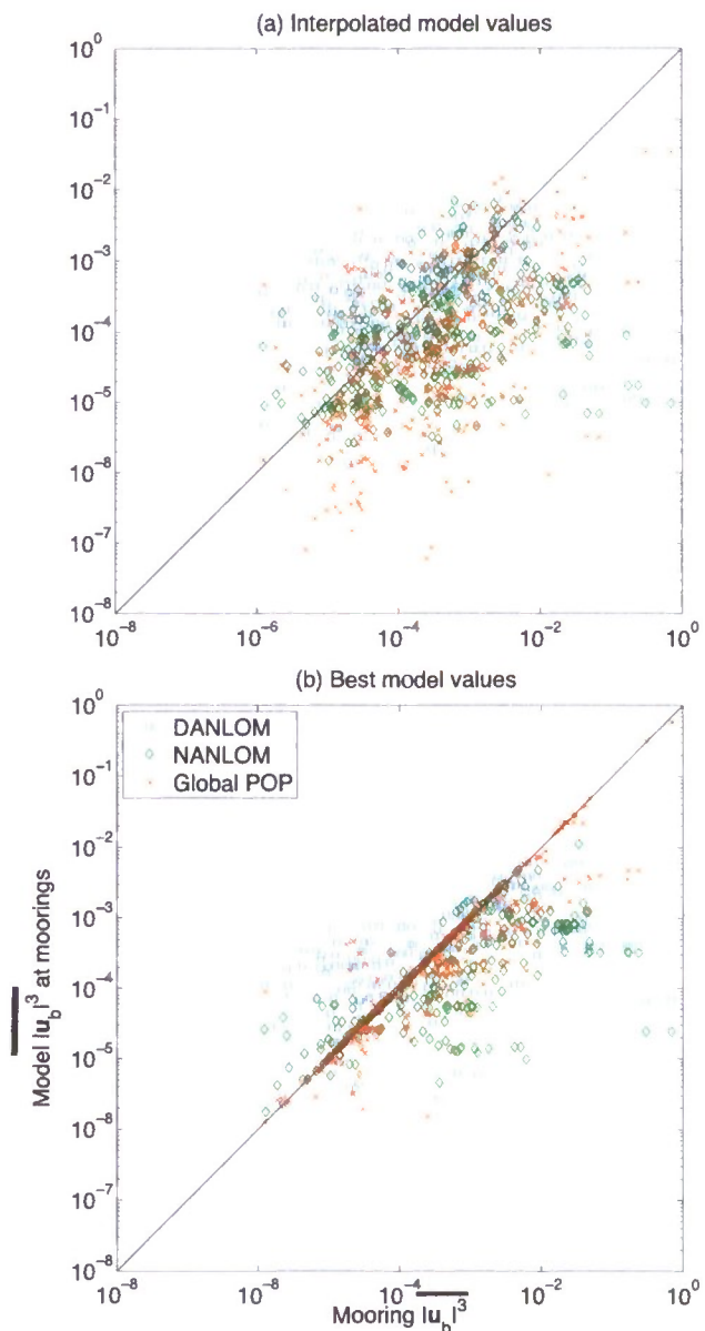
Figure 8. As in Figure 4 except that the comparison is global. Only the three global simulations are shown. All 382 near-bottom current meters in the global database are used.
