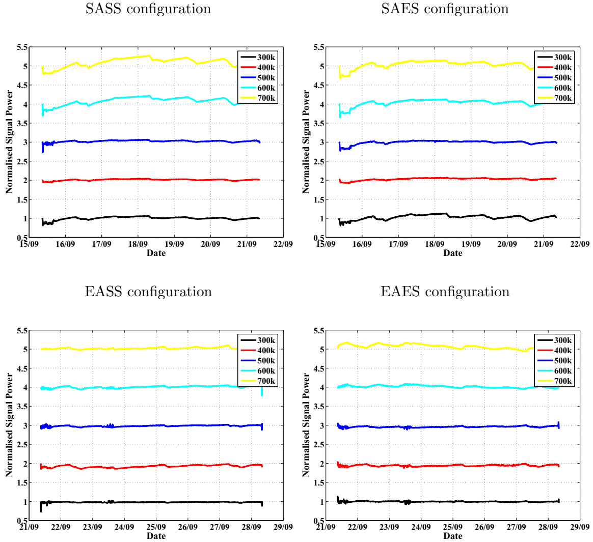
Figure A1: Variation in signal power over time for unpatched aluminium plate; Measurements for each frequency normalised to initial signal power and shifted by unity.
