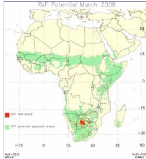
Figure 28. Rift Valley fever risk map for Africa, March 2008.
