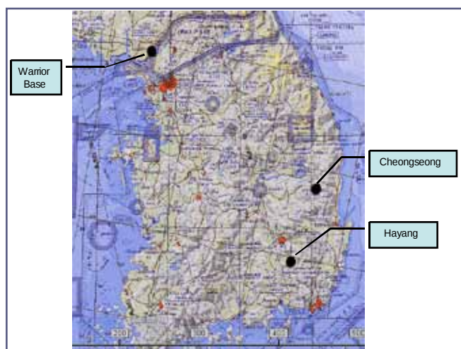
Figure 25. Primary mosquito larval collection sites in South Korea during 2007.
