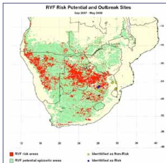
Figure 29. Summary Rift Valley fever risk map, September 2007–May 2008.
