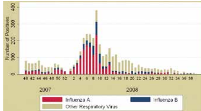
Figure 16. Positive viral results by week and year, influenza seasonal year 2007–2008.
