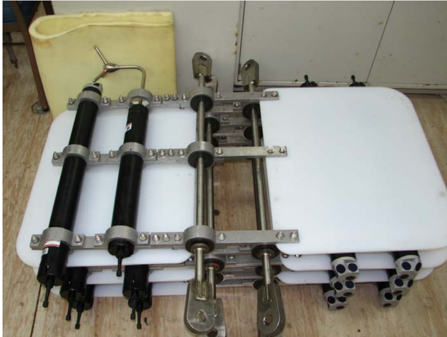
Figure 3-5: Picture of the vane system on Aquadopp HR profiler and one Vector ADV.
