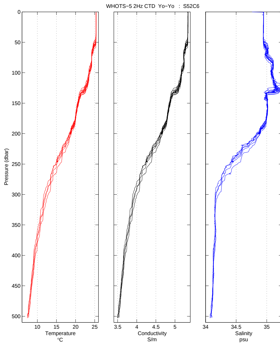
Figure A4-7. Profiles of 2 Hz temperature, conductivity and salinity data during CTD S52C6.
