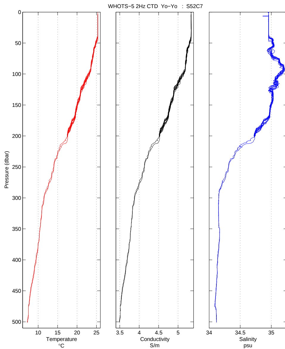
Figure A4-8. Profiles of 2 Hz temperature, conductivity and salinity data during CTD S52C7.
