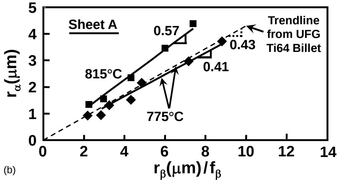
Figure 11. Static-coarsening measurements for Ti-6Al-4V Sheet A: (a) Cube of the average alpha-particle size as a function of time and (b) relationship between the alpha-particle size and the beta grain size. The results in (b) are compared to previous observations of the static coarsening behavior of an ultrafine Ti-6Al-4V billet material [16].
