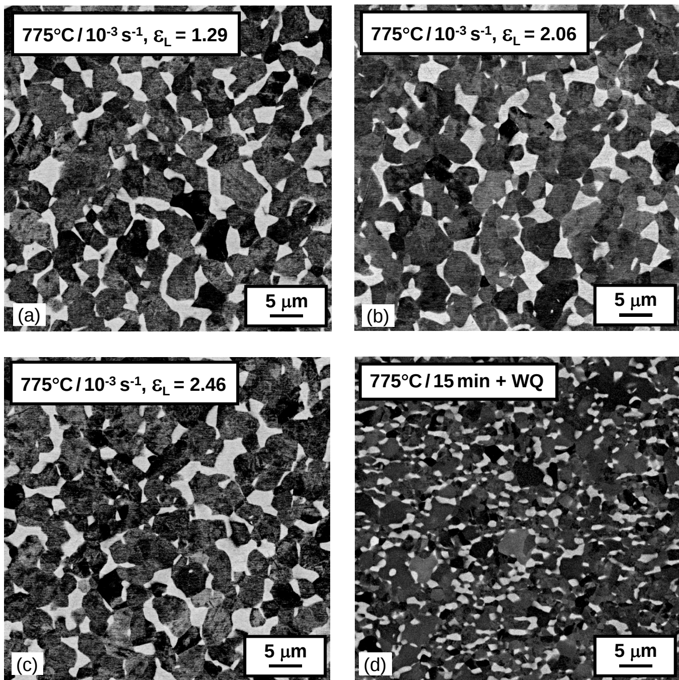
Figure 8. BSEI micrographs of Ti-6Al-4V Sheet A following tension testing at 775^{\circ}\text{C} , 10^{-3} \text{ s}^{-1} . The micrographs were taken at local true axial strains equal to: (a) 1.29, (b) 2.06, and (c) 2.46. The degree of dynamic coarsening is illustrated by comparison with the microstructure developed during heat treatment at 775^{\circ}\text{C} for 15 minutes (followed by water quenching) shown in (d).
