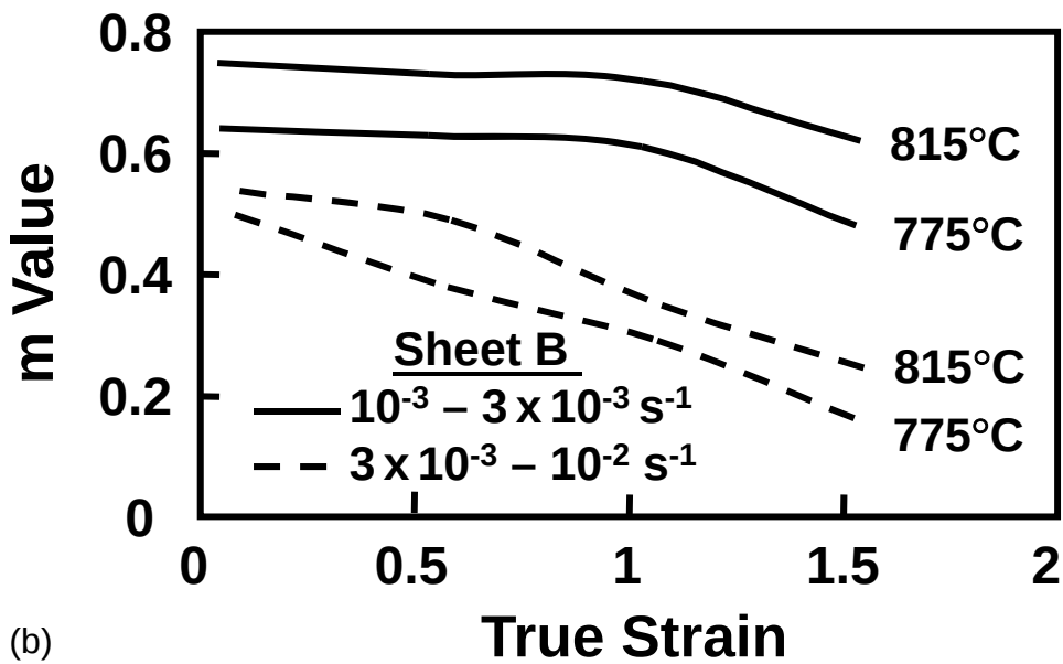
Figure 6. Strain dependence of the m value determined from jump tests at the indicated strain rates for (a) Sheet A and (b) Sheet B.
