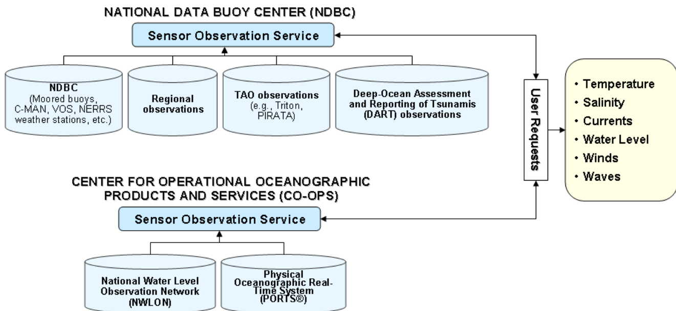
Figure 3 - Conceptual illustration of initial SOS implementation target at NDBC and CO-OPS
