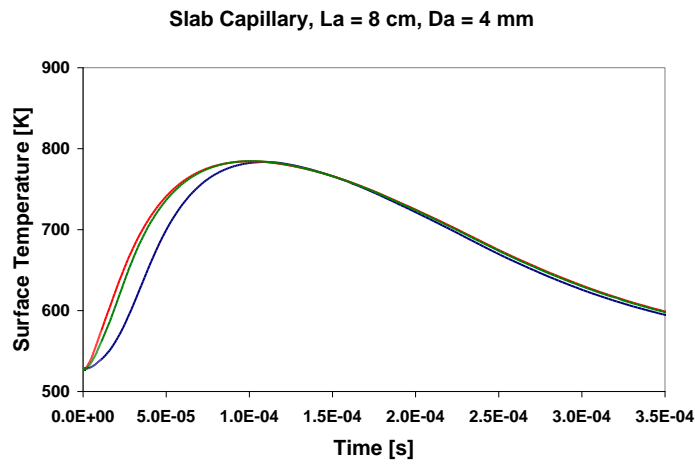
Fig. 5. Temperature of the ablative surface: blue - \eta = 0.5\text{mm} , green - \eta = 0.1\text{mm} , red - \eta = 0.02\text{mm}
