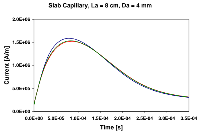
Fig.9. Current: blue - \eta = 0.5\text{mm} , green - \eta = 0.1\text{mm} , red - \eta = 0.02\text{mm}
