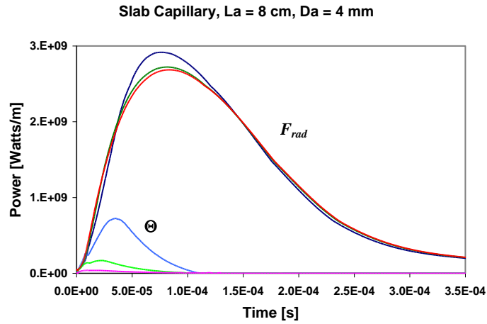
Fig. 10. F_{rad} and \Theta : blue and light blue - \eta = 0.5\text{mm} , green and light green - \eta = 0.1\text{mm} , red and pink - \eta = 0.02\text{mm} .
