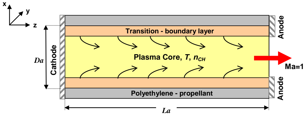
Fig. 1: Schematic (not to scale) of slab capillary discharge operation; (x, z) cross section is shown
