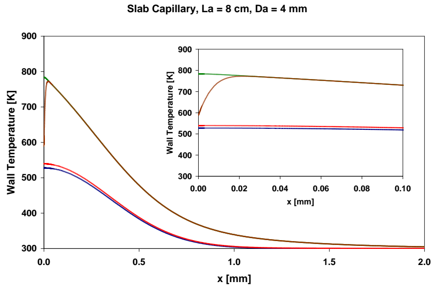
Fig. 13. Wall temperature distribution: \eta = 0.5 \mu\text{m} , blue - 0 sec, red - 11 \mu\text{s} , green – 111 \mu\text{s} , brown – 361 \mu\text{s} .
