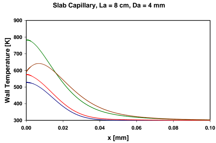
Fig. 11. Wall temperature distribution: \eta = 0.02 \mu\text{m} , blue - 0 sec, red - 11 \mu\text{s} , green - 111 \mu\text{s} , and brown - 361 \mu\text{s} .
