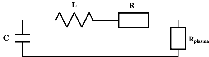
Fig. 2 RLC circuit for modeling capillary discharge.
