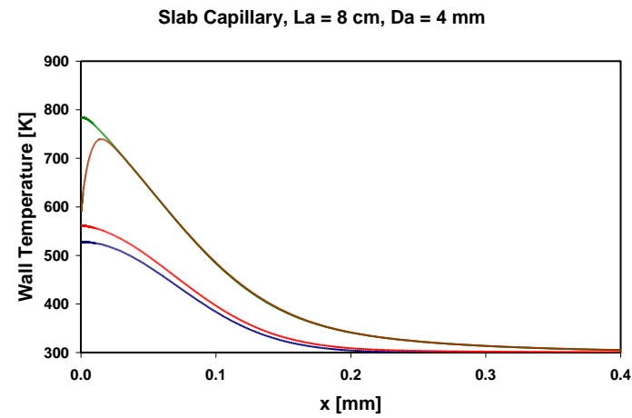
Fig. 12. Wall temperature distribution: \eta = 0.1 \mu\text{m} , blue - 0 sec, red - 11 \mu\text{s} , green - 111 \mu\text{s} , and brown - 361 \mu\text{s} .
