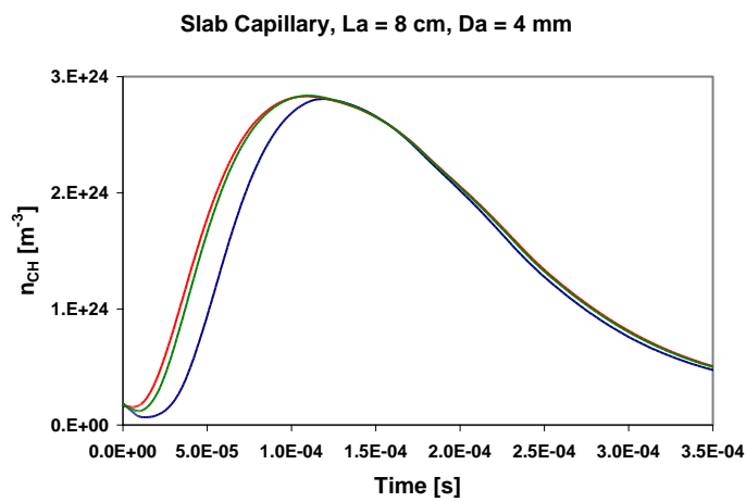
Fig. 6. Polyethylene number density in the plasma core region: blue - \eta = 0.5\text{mm} , green - \eta = 0.1\text{mm} , red - \eta = 0.02\text{mm}
