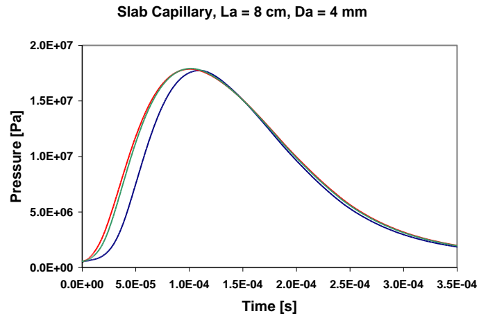
Fig. 7. Plasma pressure: blue - \eta = 0.5\text{mm} , green - \eta = 0.1\text{mm} , red - \eta = 0.02\text{mm}
