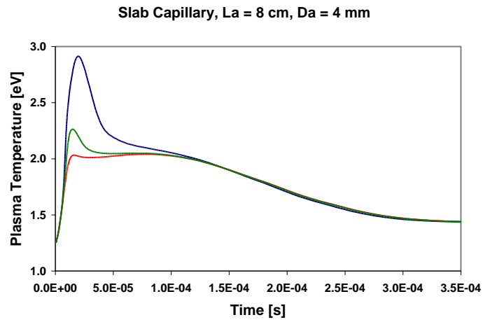
Fig. 8. Plasma temperature: blue - \eta = 0.5\text{mm} , green - \eta = 0.1\text{mm} , red - \eta = 0.02\text{mm}
