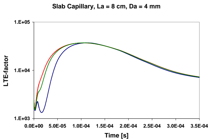
Fig. 3. LTE-factor: blue - \eta = 0.5 mm, green - \eta = 0.1 mm, red - \eta = 0.02 mm
