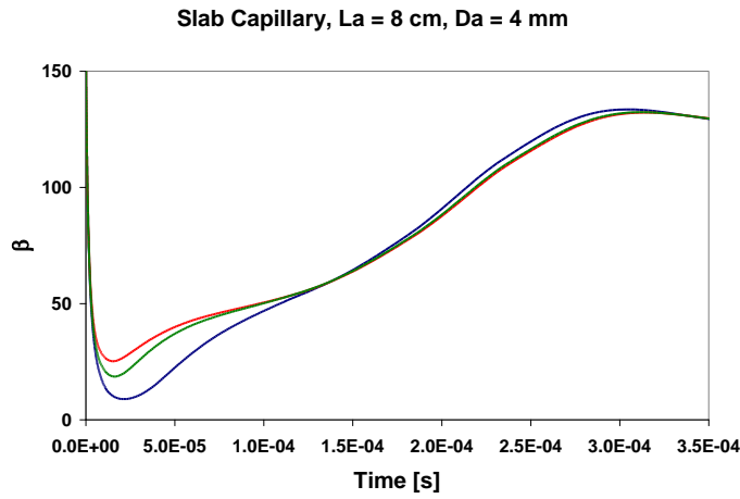
Fig. 4. \beta : blue - \eta = 0.5\text{mm} , green - \eta = 0.1\text{mm} , red - \eta = 0.02\text{mm}
