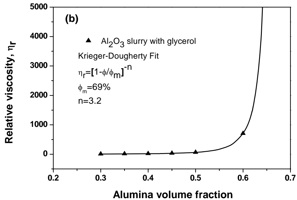
Fig. 3 Relative viscosity at a shear rate of 100 \text{ s}^{-1} as a function of volume fraction for alumina slurries with and without glycerol
