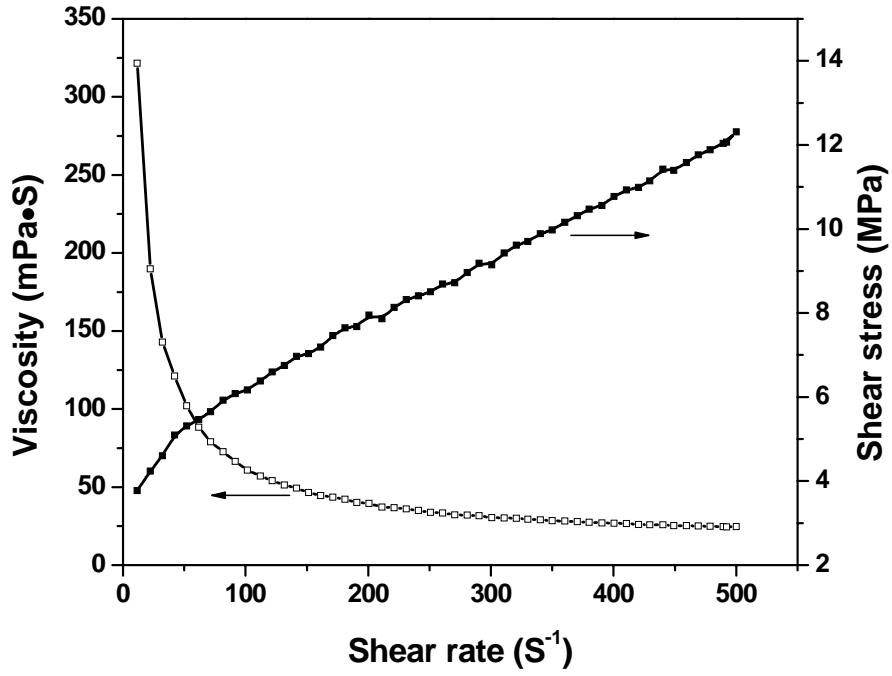
Fig. 2 Rheological behavior of 45vol% Al 2 O 3 slurry with glycerol
