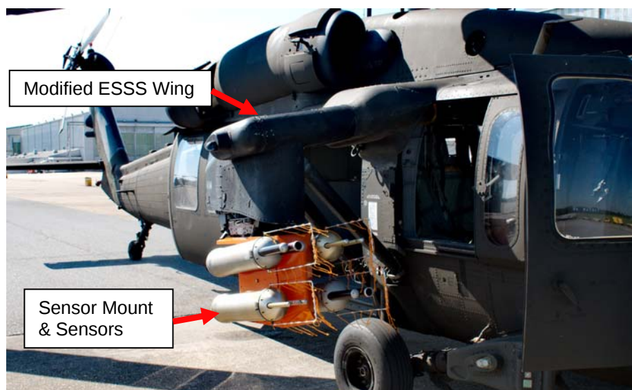
Figure 3. UH-60M Configured for Icing Tests
