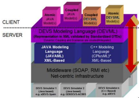
Figure 5: DEVS Transparency and Net-centric model interoperability using DEVSMML. Client and Server categorization is done for DEVS/SOA implementation
