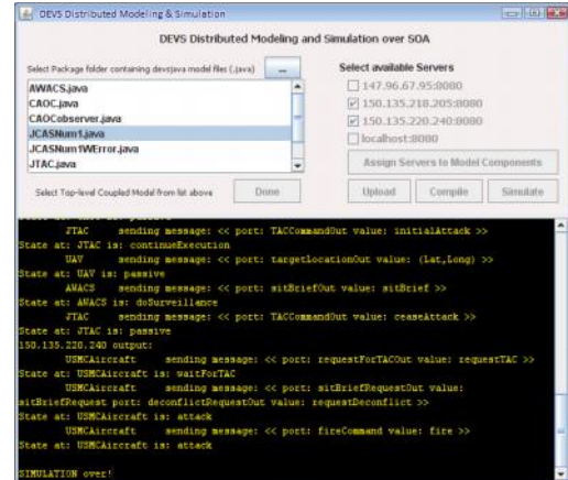
Figure 7: GUI snapshot of DEVJS/SOA client hosting distributed simulation
