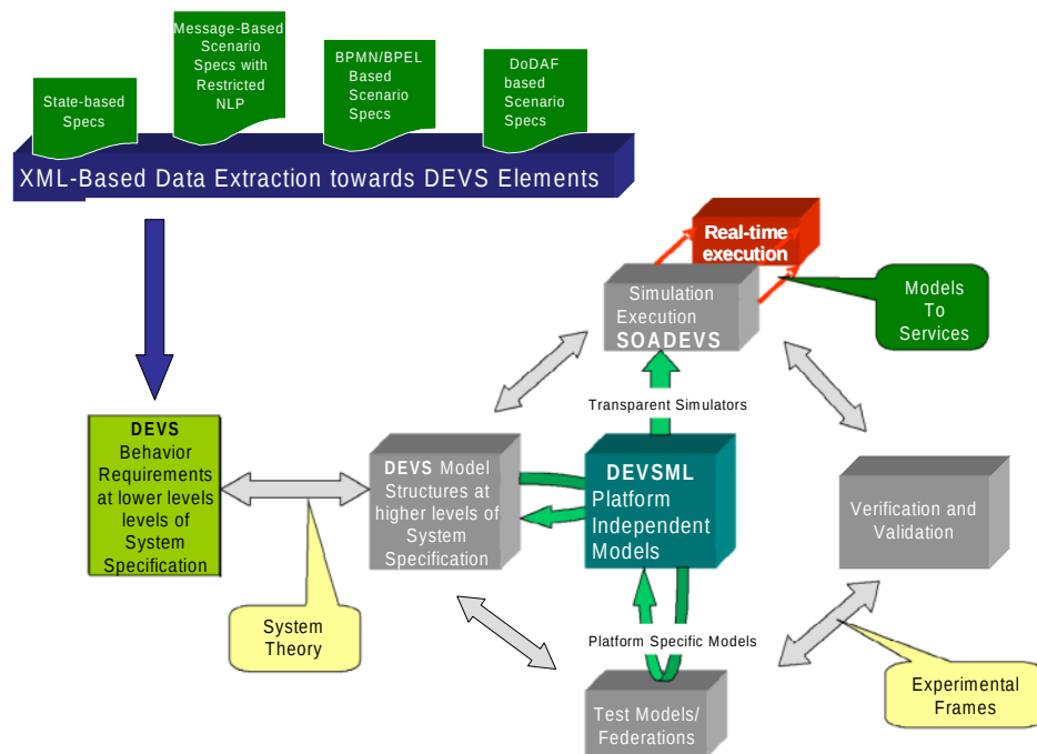
Figure 9: The Complete DEVS Unified Process
