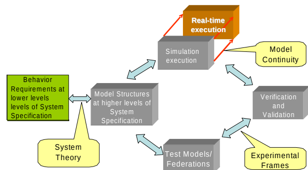
Figure 3: Bifurcated Model-Continuity based System Life-cycle Process
