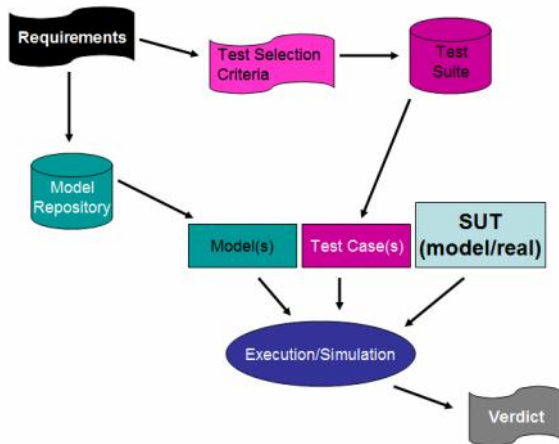
Figure 1: Graphical process extended further from [Utt06]
