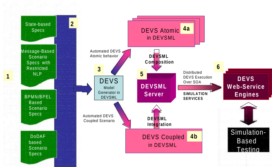
Figure 4: Net-centric collaboration and execution using DEVSMML and DEVS/SOA
