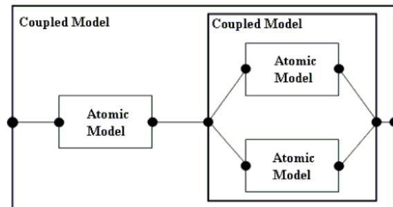
Figure 2: DEVS atomic and coupled models
