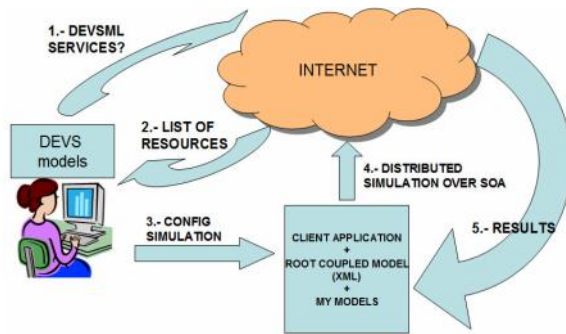
Figure 6: Execution of DEVS SOA-Based M&S
