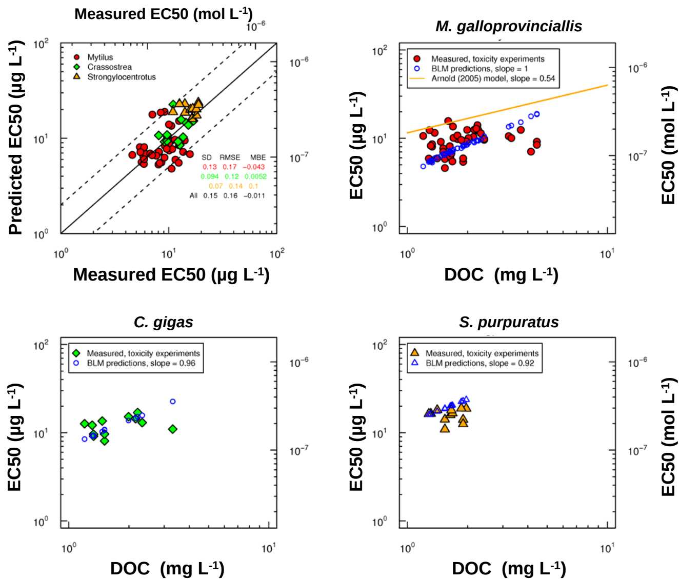
Figure 79. Measured and predicted Cu diss EC50s for Pearl Harbor.
