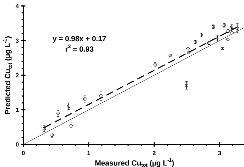
Figure 26. Predicted versus measured \text{Cu}_{\text{tot}} ( \mu\text{g L}^{-1} ) for 30 August 2000 (SD26). Measured \text{Cu}_{\text{tot}} from SERDP CP-1156 and predicted daily mean ( \circ , with \pm 1 sd) by the integrated CH3D/seawater-BLM model, with regression (broken line). The solid line is the one-to-one ratio. The same symbol and lines are used in the corresponding figures below.
