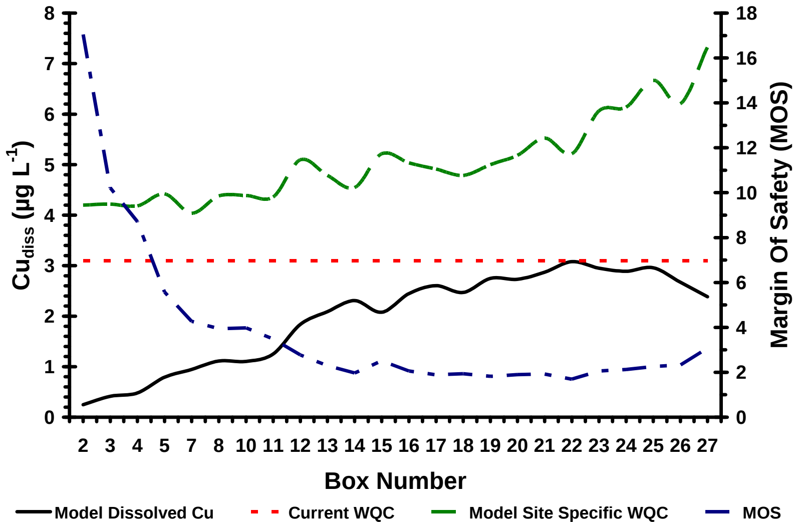
Figure 84. Relief predicted by the integrated CH3D/seawater-BLM model with a site-specific WQC for San Diego Bay. The MOS is the \times -fold increase in \text{Cu}_{\text{diss}} required to reach the toxicity threshold.
