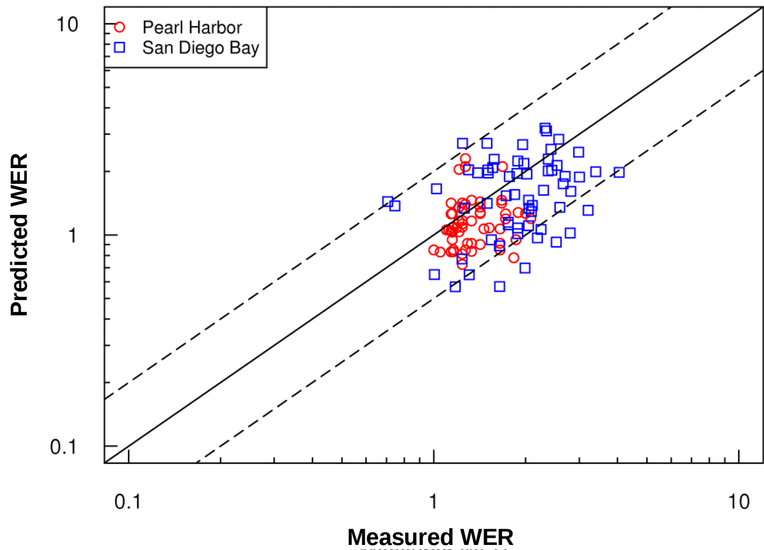
Figure 83. Comparison between WERs predicted by the integrated model and measured in San Diego Bay and Pearl Harbor.
