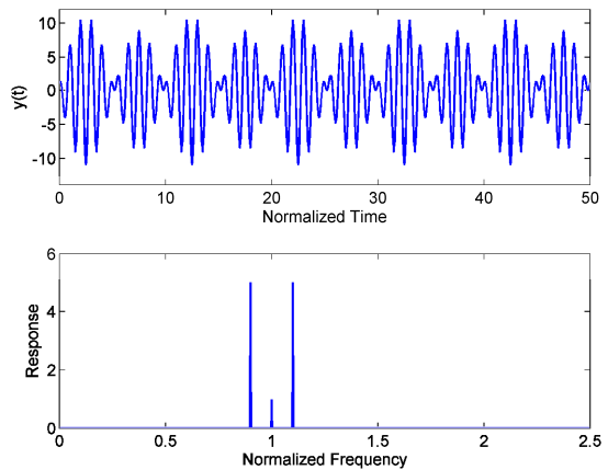
Figure 6 Amplitude modulation with \beta > 1
