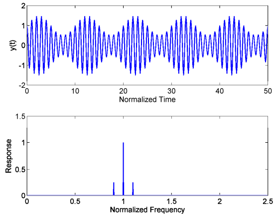
Figure 5 Amplitude modulation with \beta < 1
