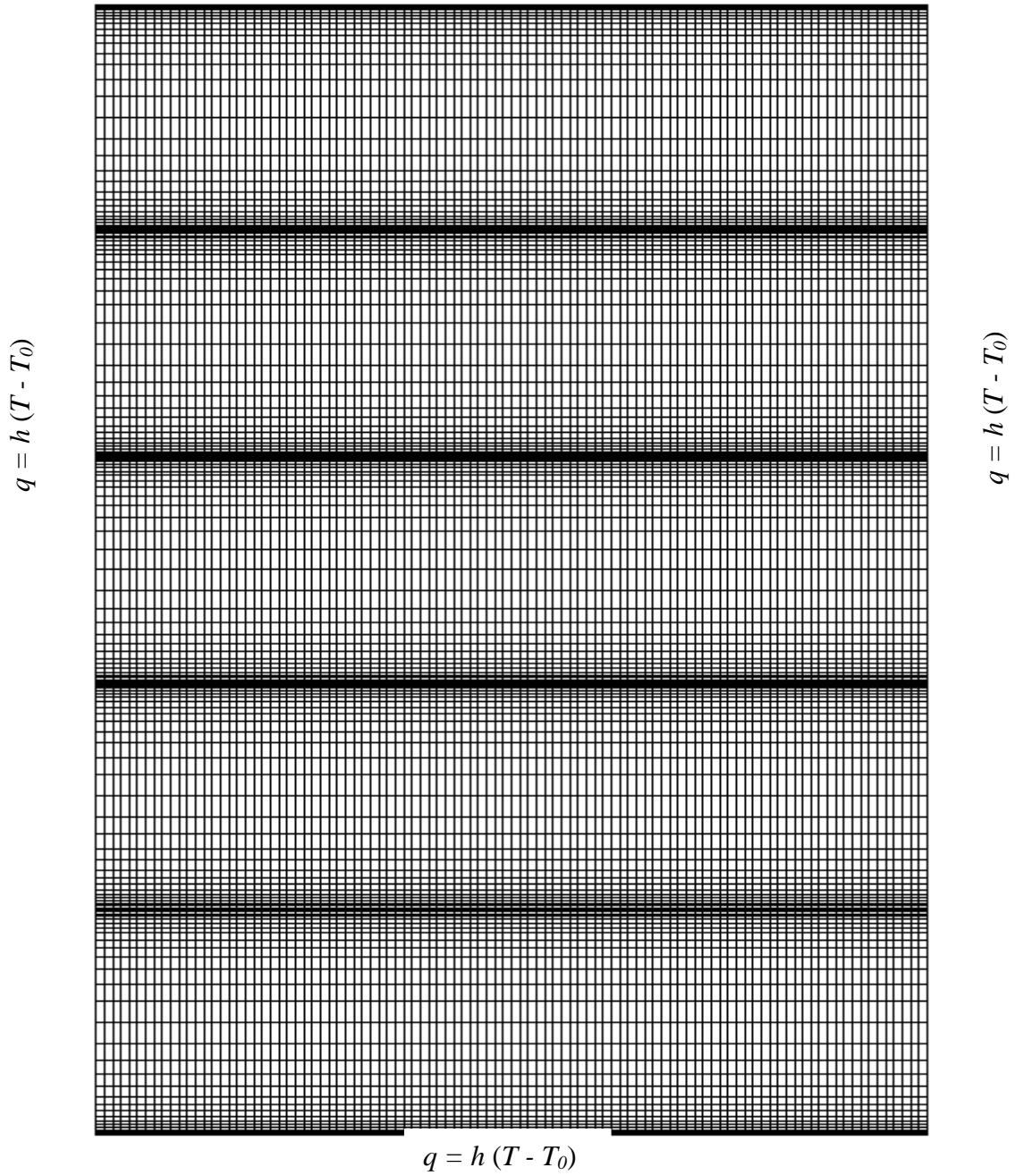
Figure 3. Finite element mesh of the multidisk clutch.
