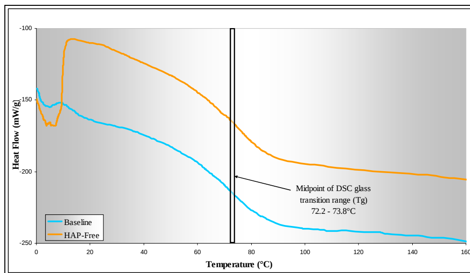
Figure 9. Torque Seal DSC.
