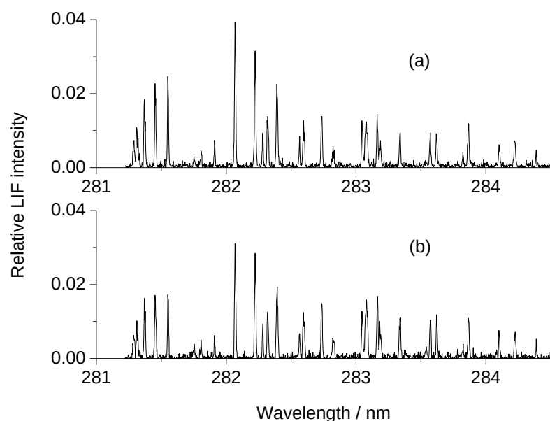
Fig. 7 Representative OH A-X (1,0) excitation spectra from [DMIM] [Im]. (a) Thermal spectrum recorded at a photolysis-probe laser delay of 30 \mu s, p(\text{NO}_2) \sim 1 mTorr and p(\text{N}_2) \sim 0.5 Torr. (b) Nascent spectrum recorded at a photolysis-probe laser delay of 8 \mu s, probe laser-liquid surface distance = 4 mm p(\text{NO}_2) \sim 1 mTorr.
